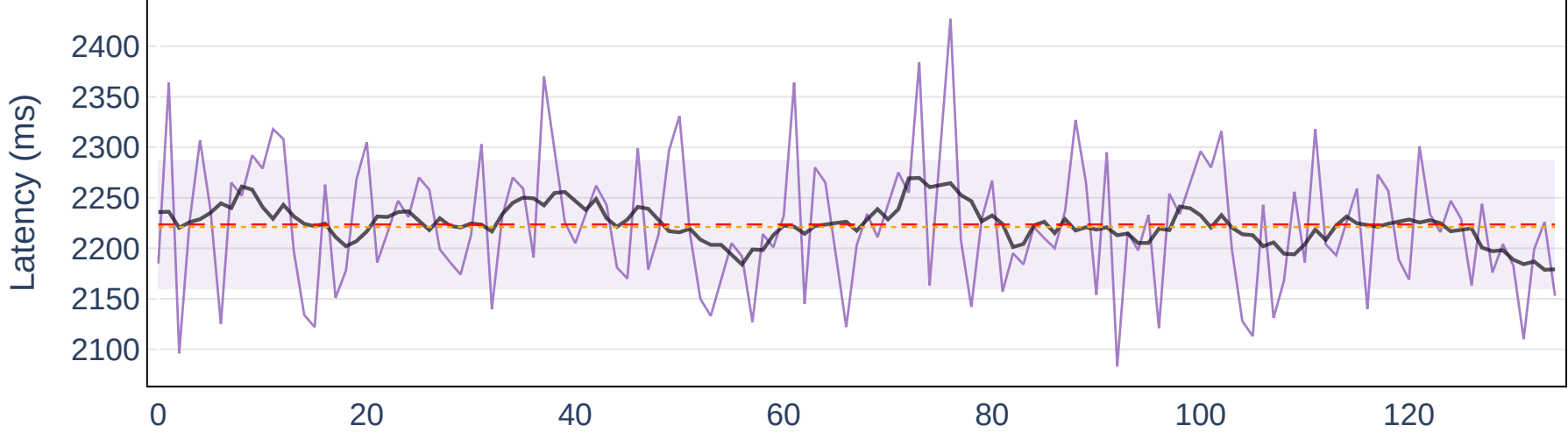
Lab, Trial 2: BPSK
