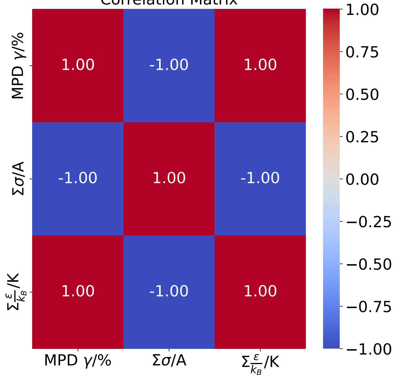
Correlation Matrix
