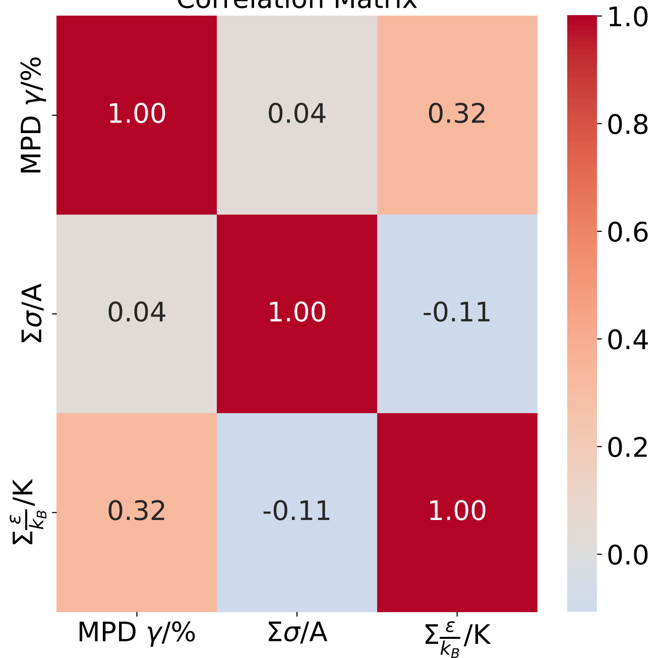
Correlation Matrix
