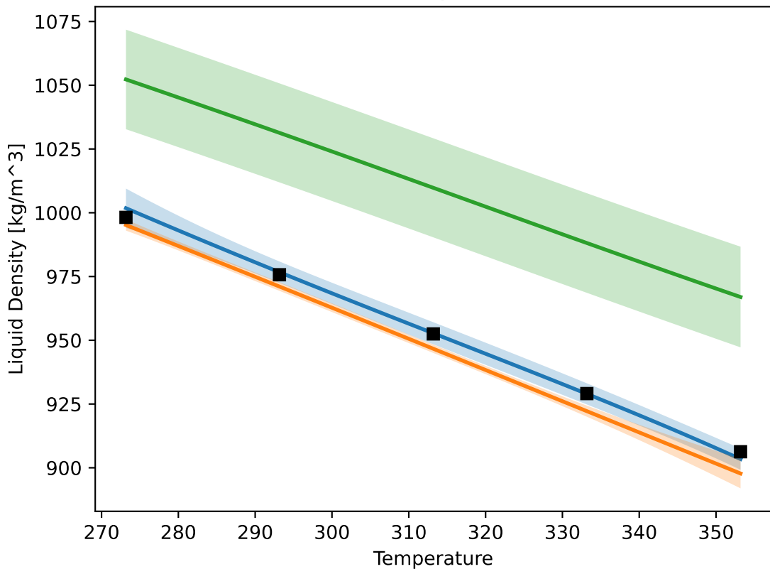
GP Model vs. Exp Data for DEC
