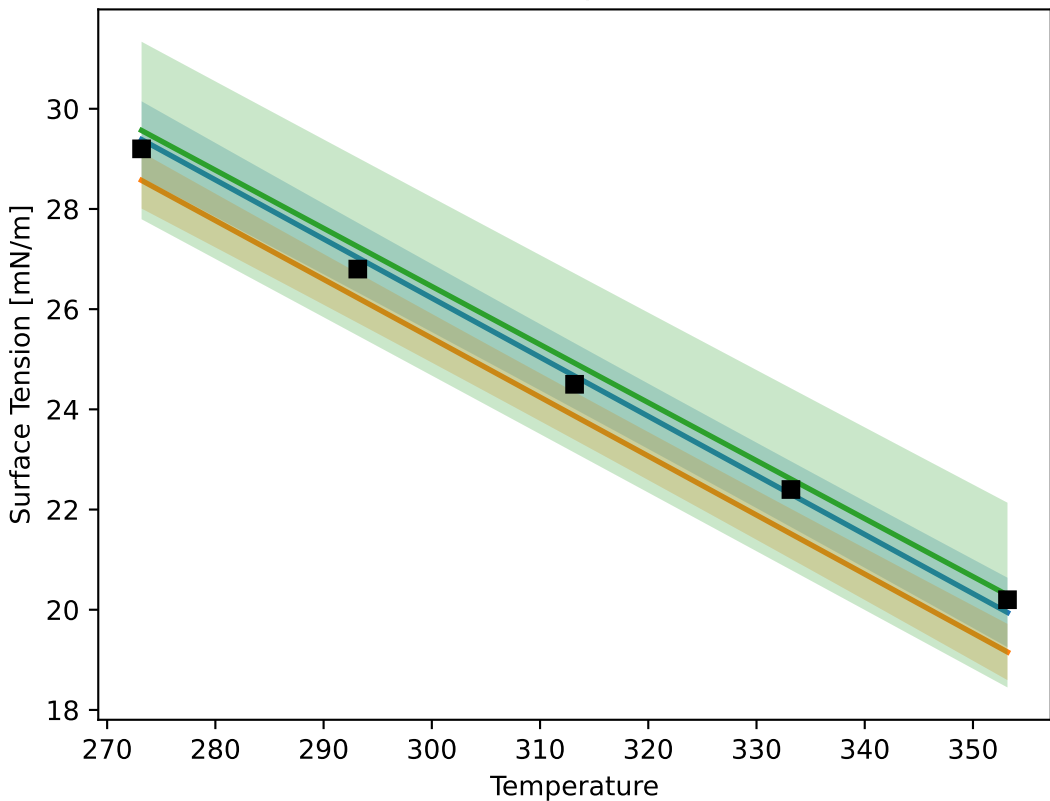
GP Model vs. Exp Data for DEC
