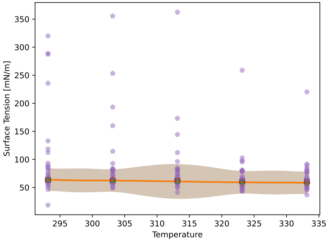
GP Model vs. Exp Data for Gly
