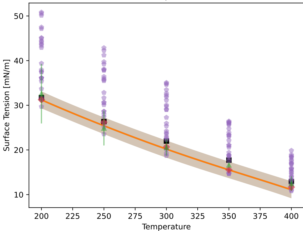
GP Model vs. Exp Data for MeOH
