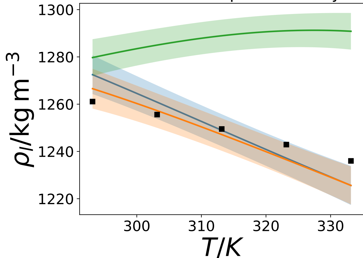
GP Model vs. Exp Data for Gly
