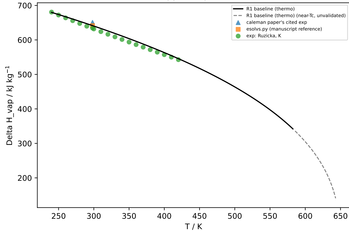
Enthalpy of vaporization
