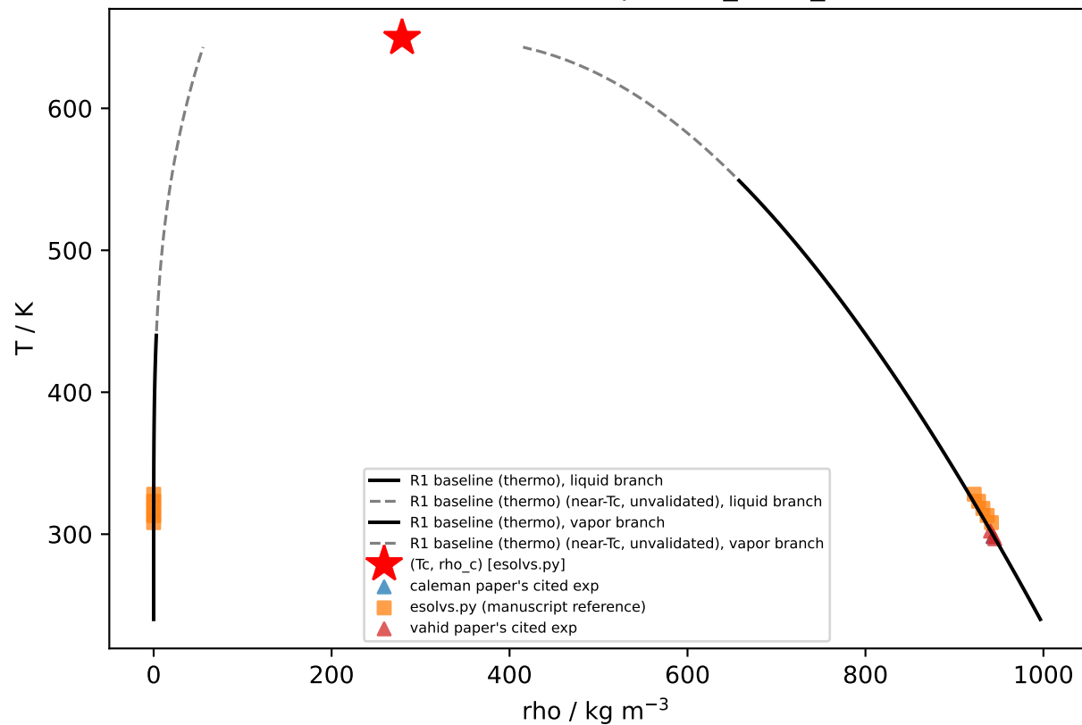
Coexistence envelope (rho_l, rho_v)
