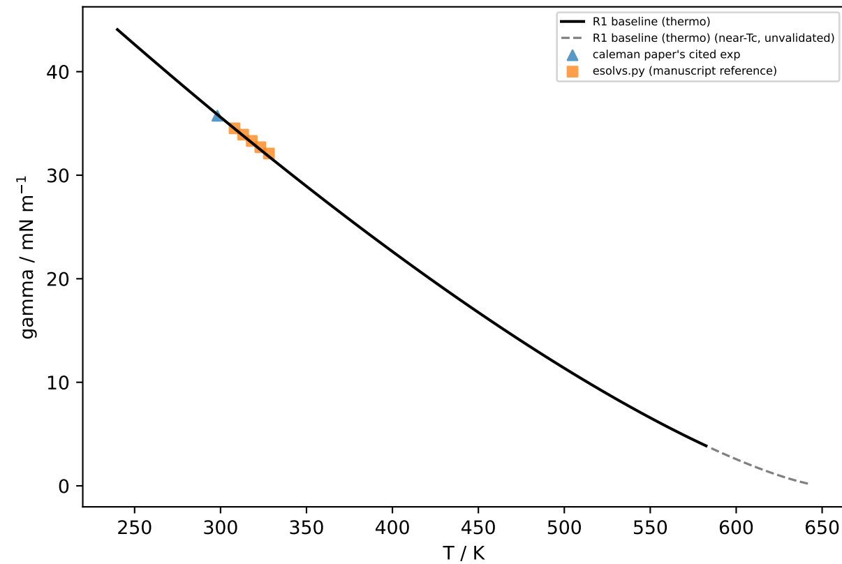
Surface tension
