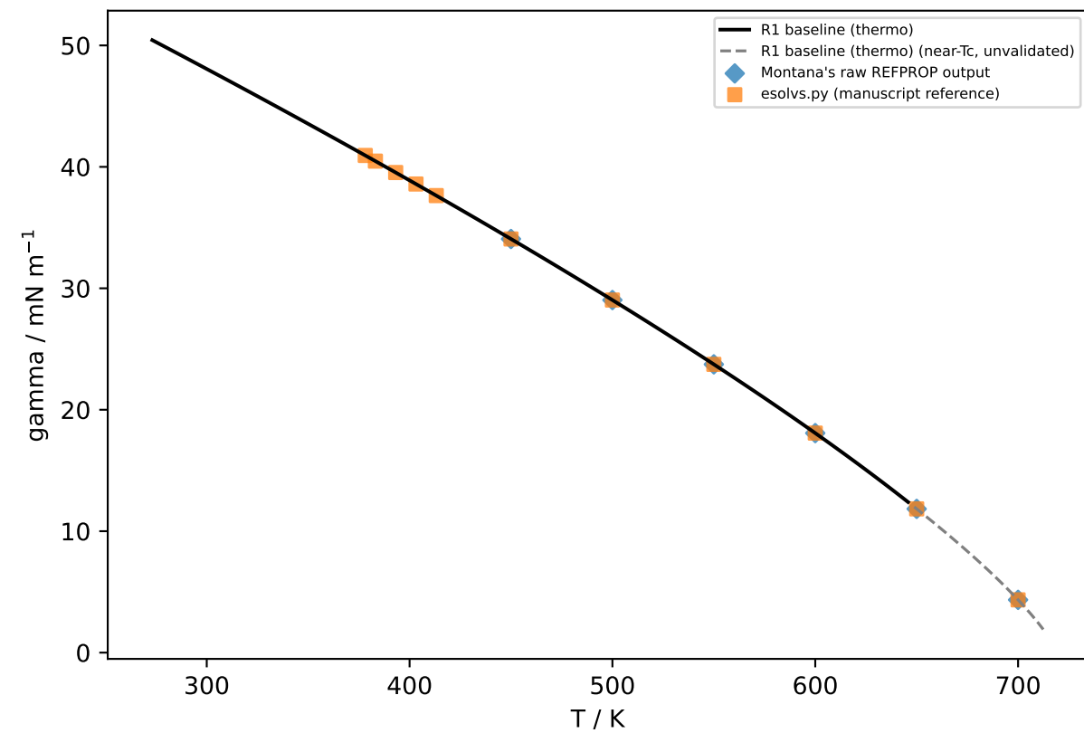
Surface tension
