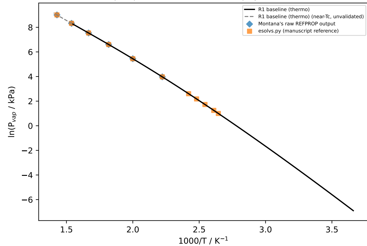
Vapor pressure (Clausius-Clapeyron axes)
