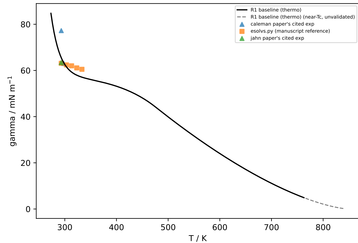
Surface tension
