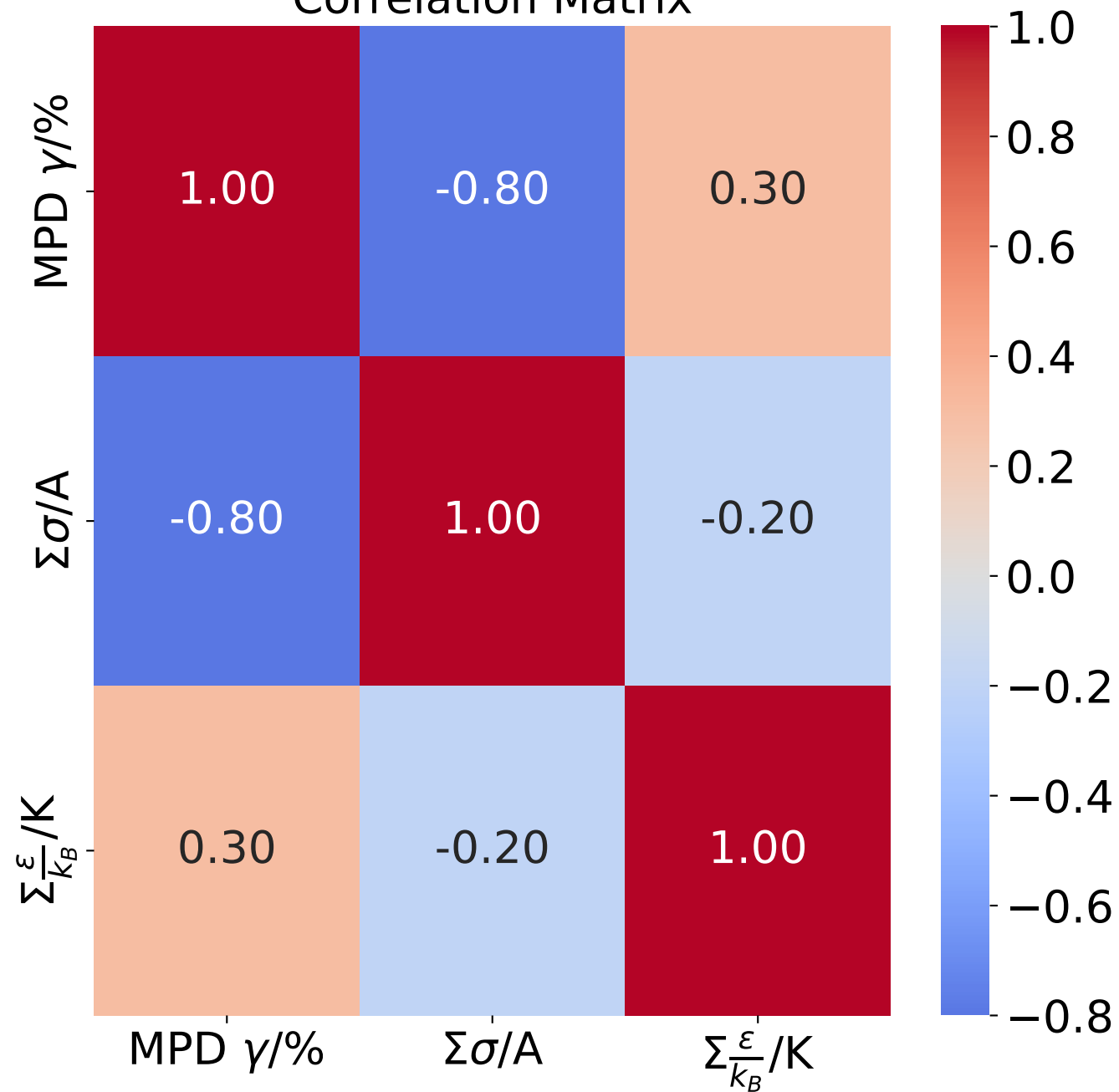
Correlation Matrix
