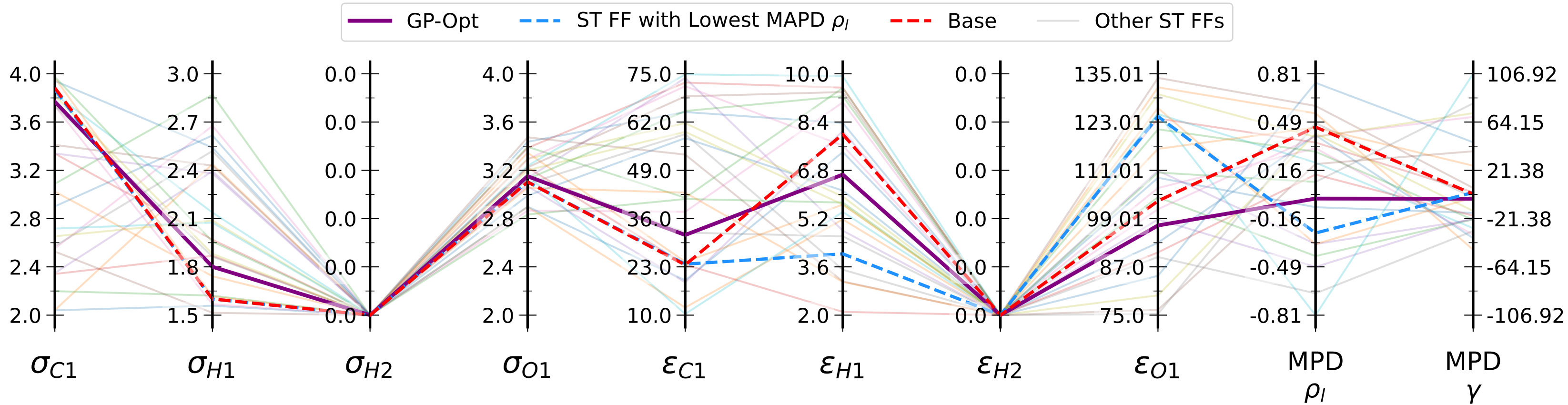
EG - Comparison of GP-Optimized FF and Unoptimized ST Iter FFs
