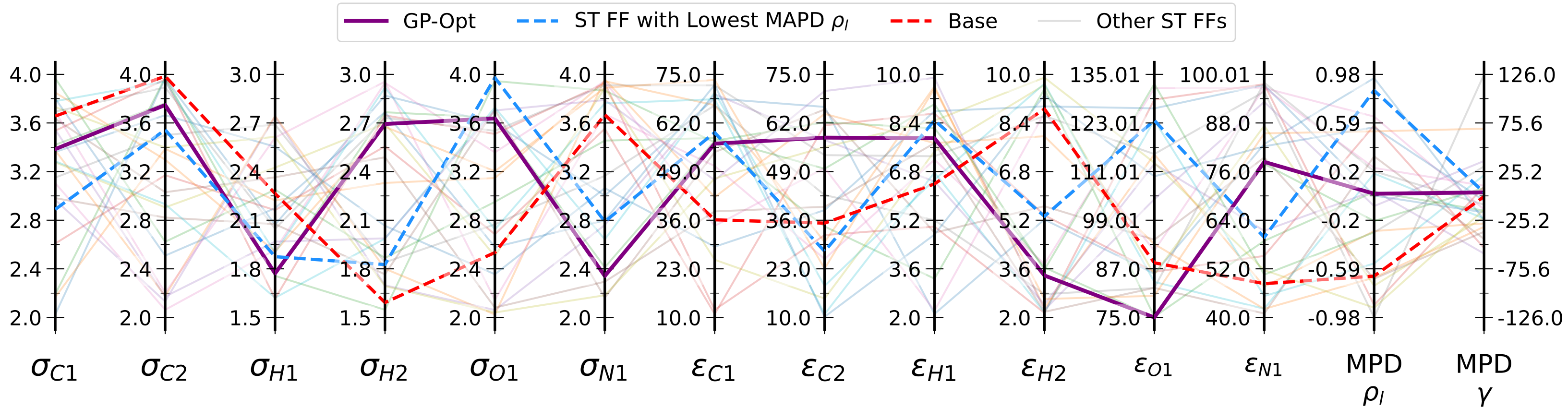
DMF - Comparison of GP-Optimized FF and Unoptimized ST Iter FFs
