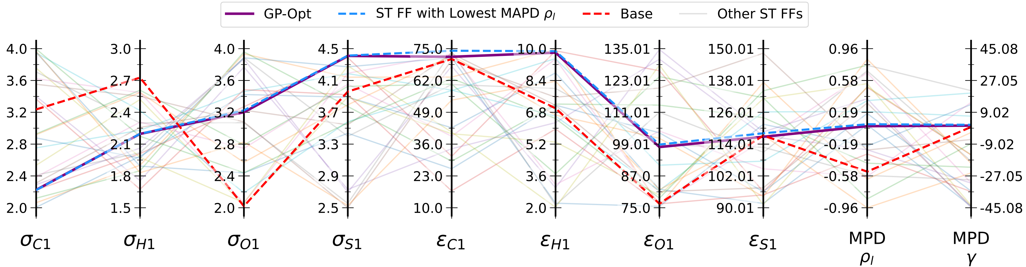
DMSO - Comparison of GP-Optimized FF and Unoptimized ST Iter FFs
