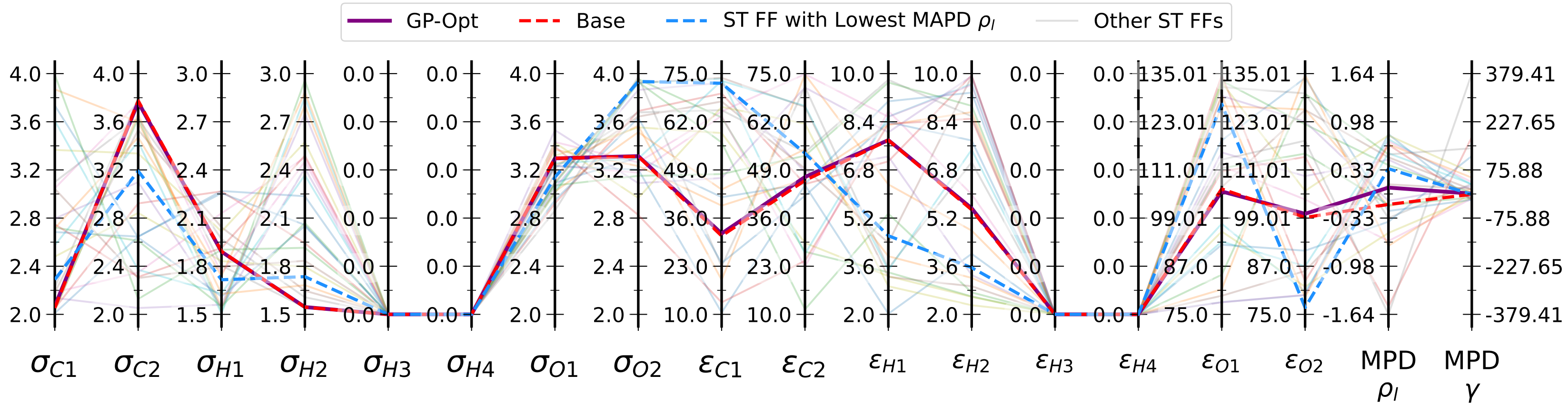
Gly - Comparison of GP-Optimized FF and Unoptimized ST Iter FFs
