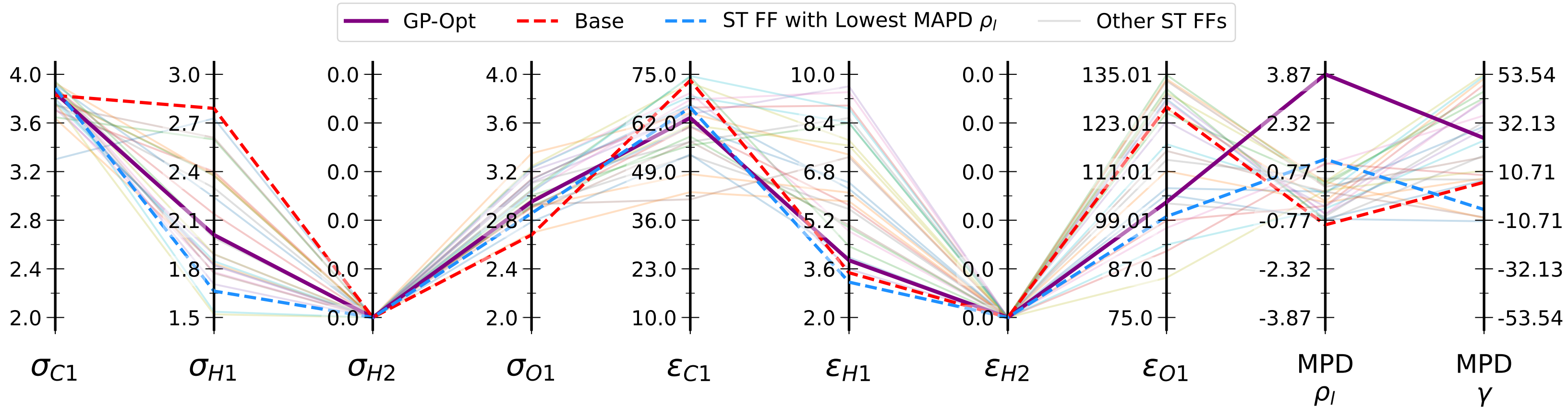
MeOH - Comparison of GP-Optimized FF and Unoptimized ST Iter FFs
