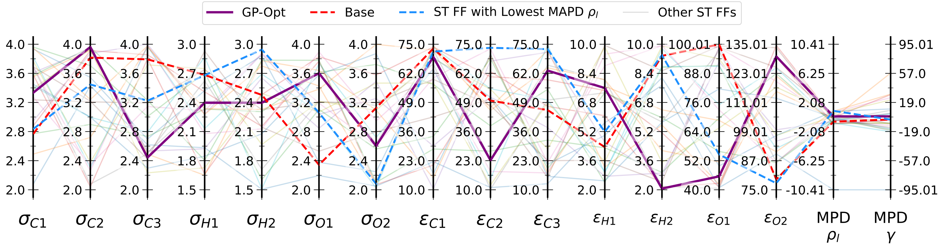
DEC - Comparison of GP-Optimized FF and Unoptimized ST Iter FFs
