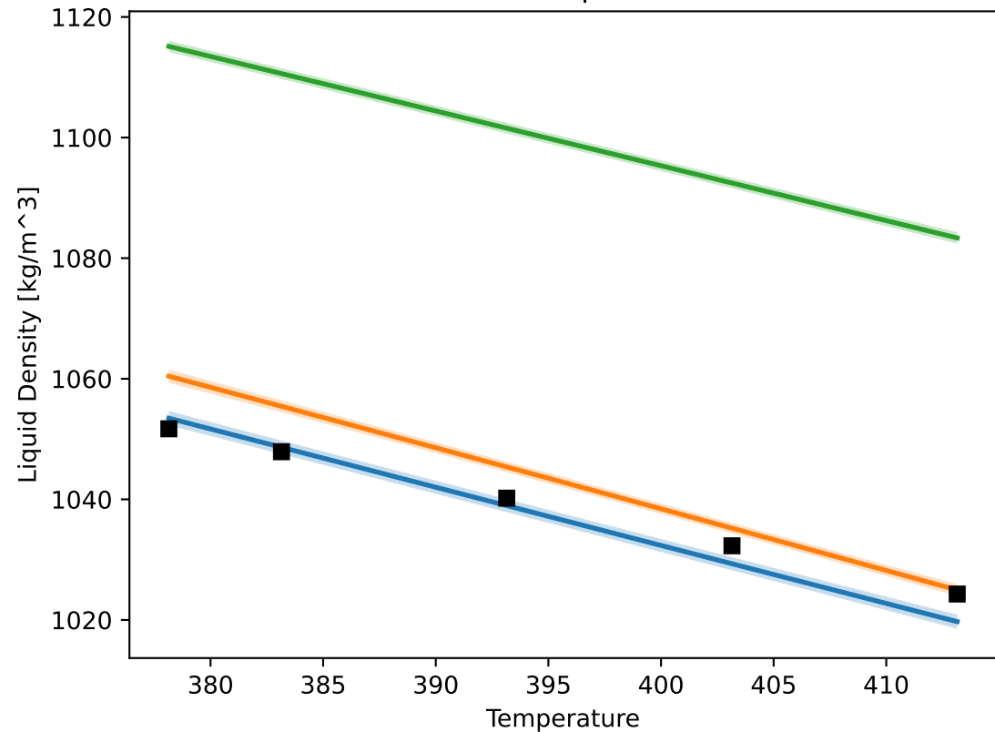
GP Model vs. Exp Data for EG
