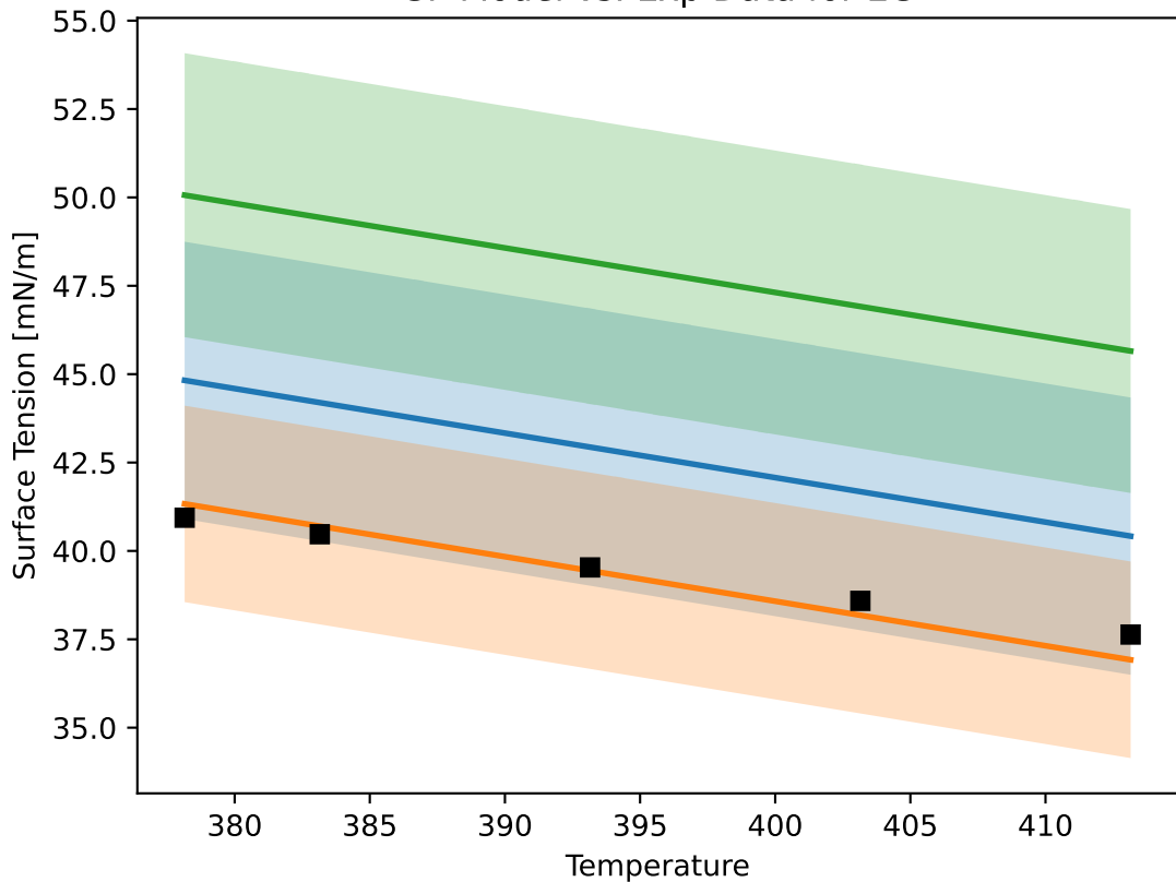
GP Model vs. Exp Data for EG
