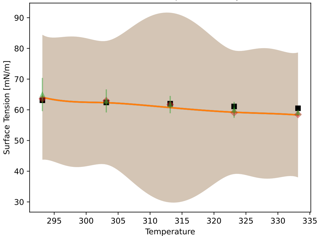
GP Model vs. Exp Data for Gly
