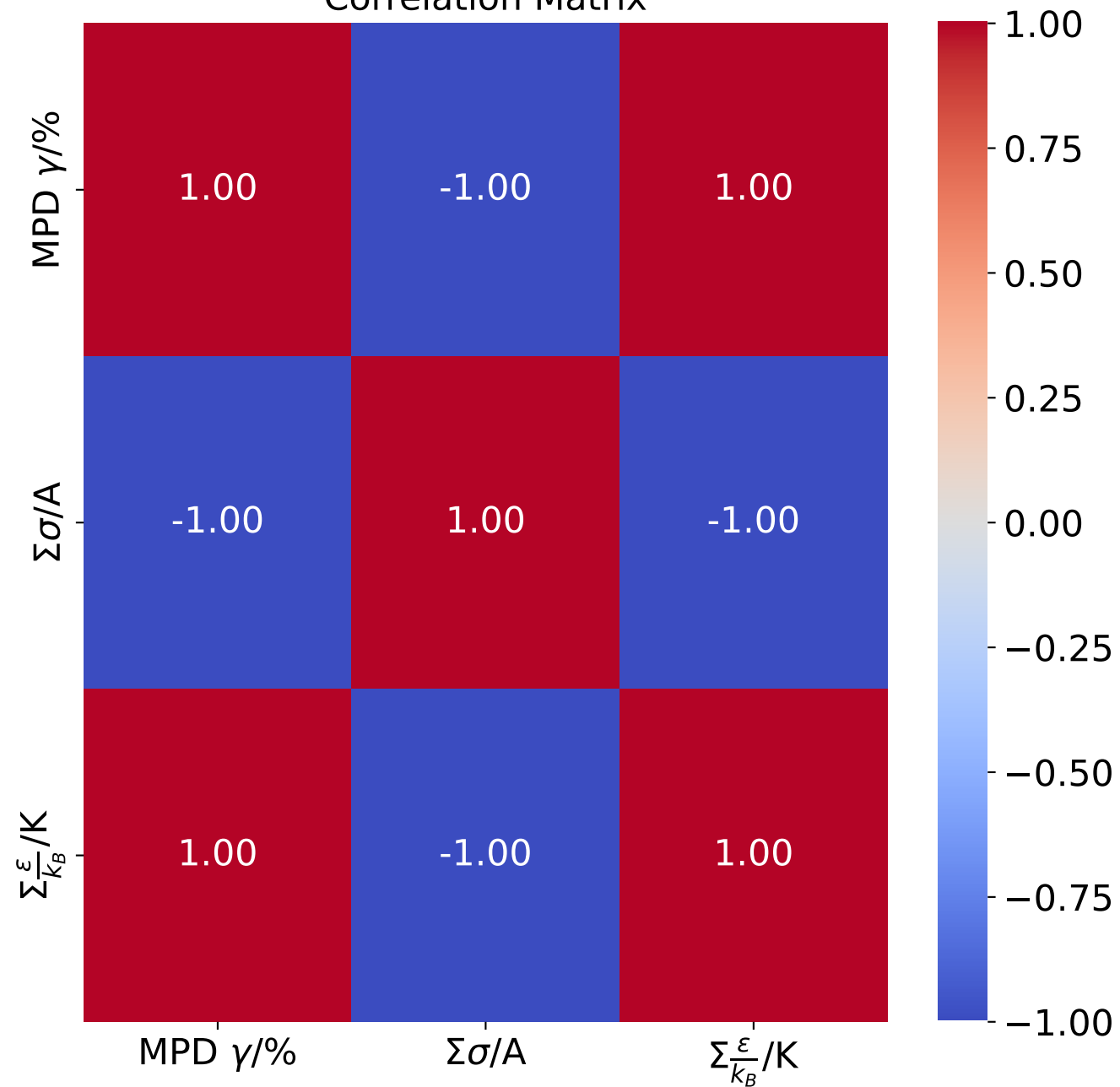
Correlation Matrix
