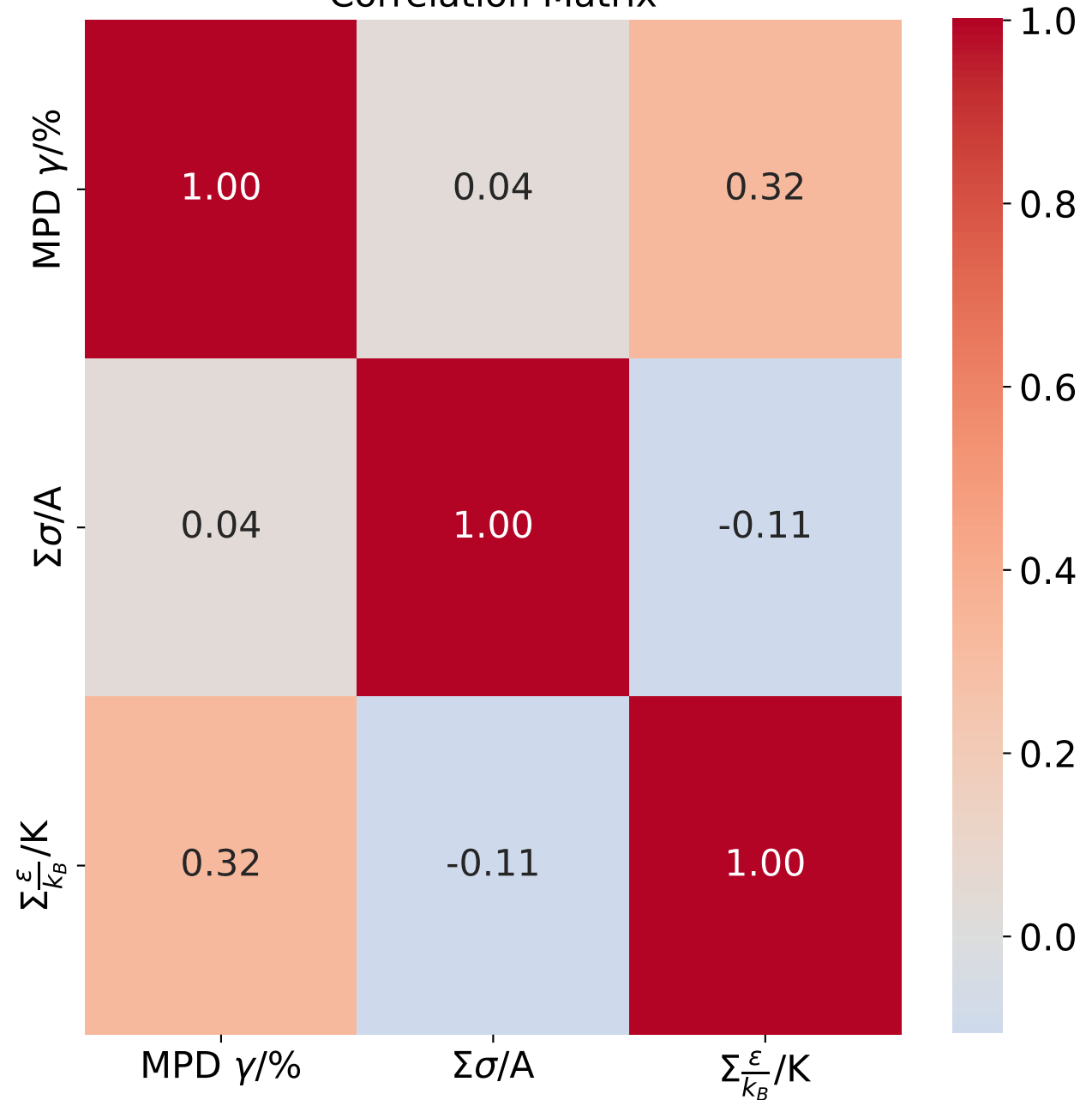
Correlation Matrix
