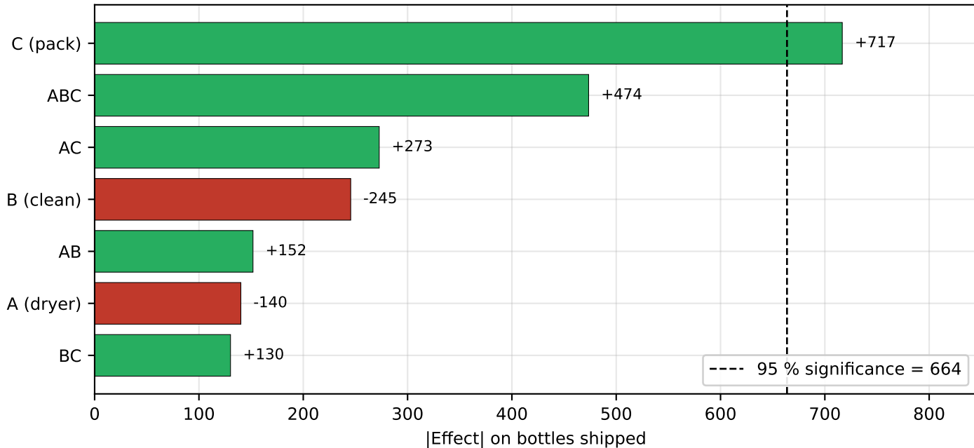
2 3 DOE Pareto of effects (dryer × clean × pack)
