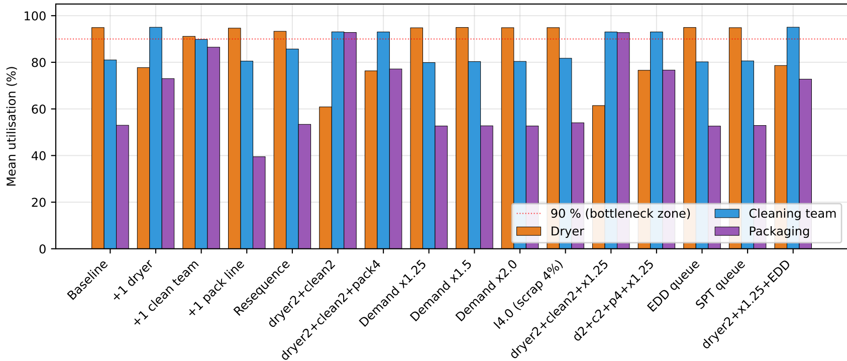
Resource utilisation by scenario — bottleneck shifts with capacity
