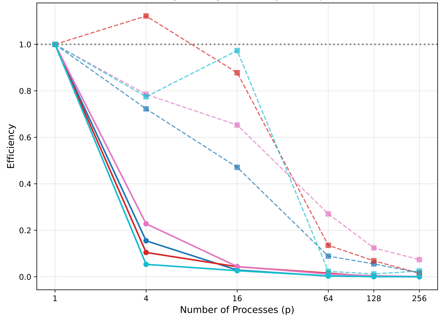
Strong Scaling: Efficiency ( E = S/p )
