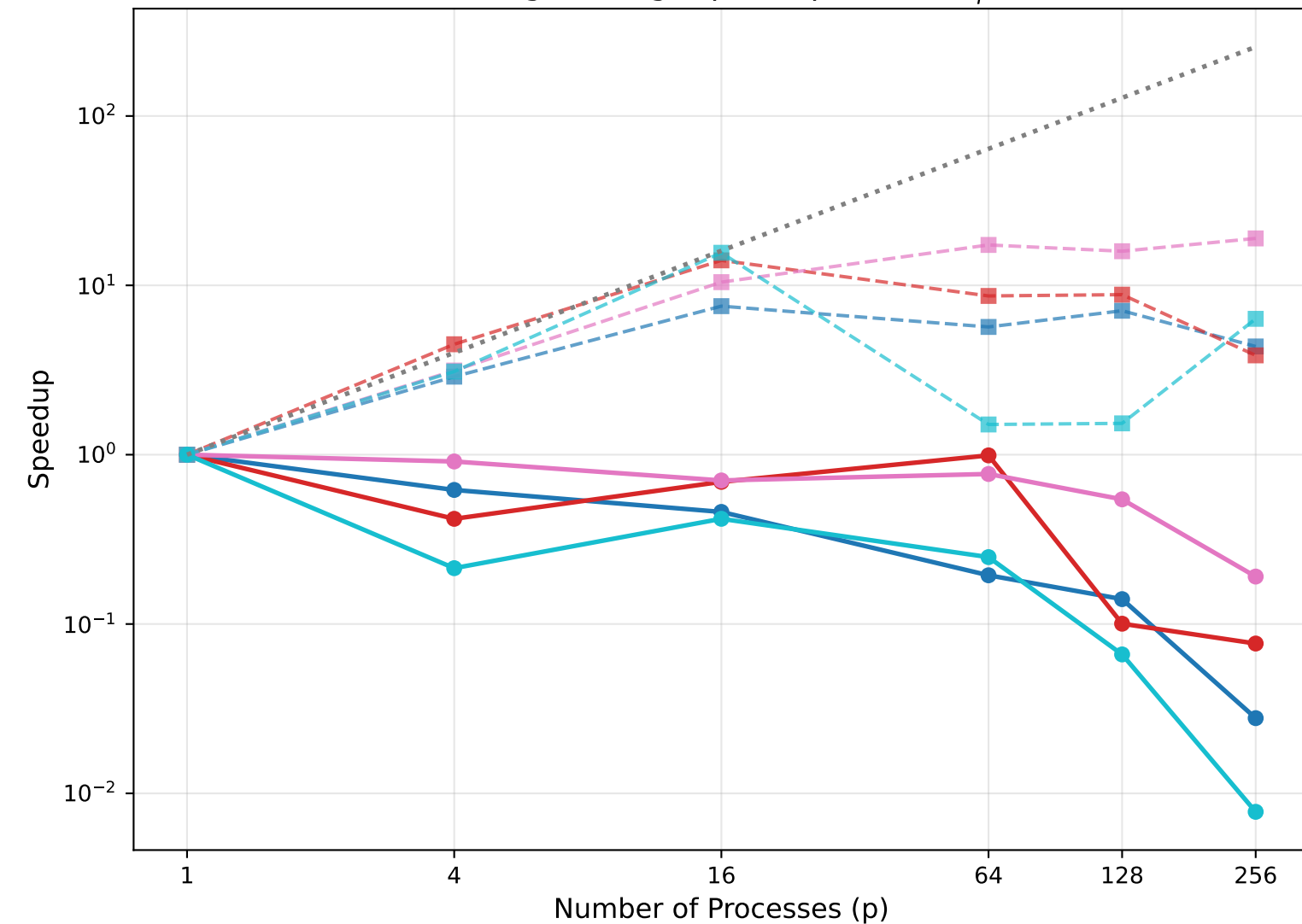
Strong Scaling: Speedup ( S = T_1/T_p )
