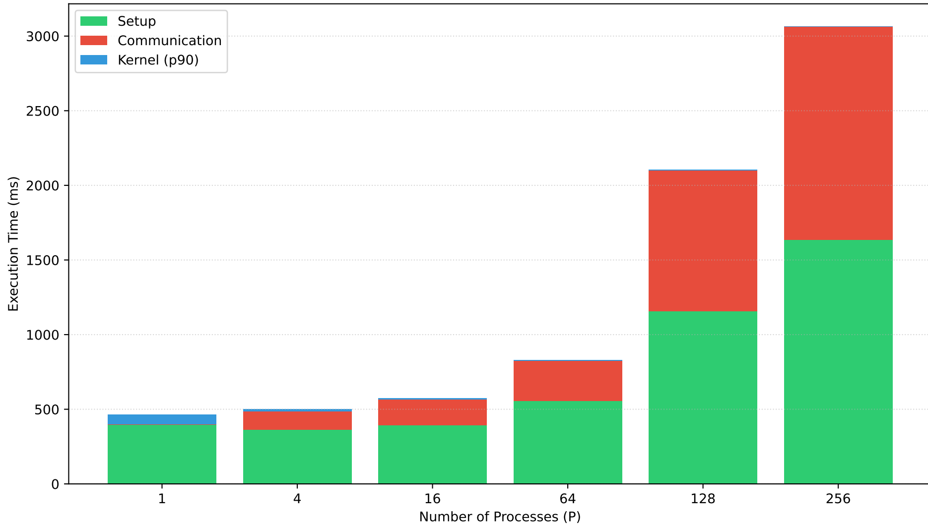
Execution Breakdown: ./matrices/cit-Patents.mtx
