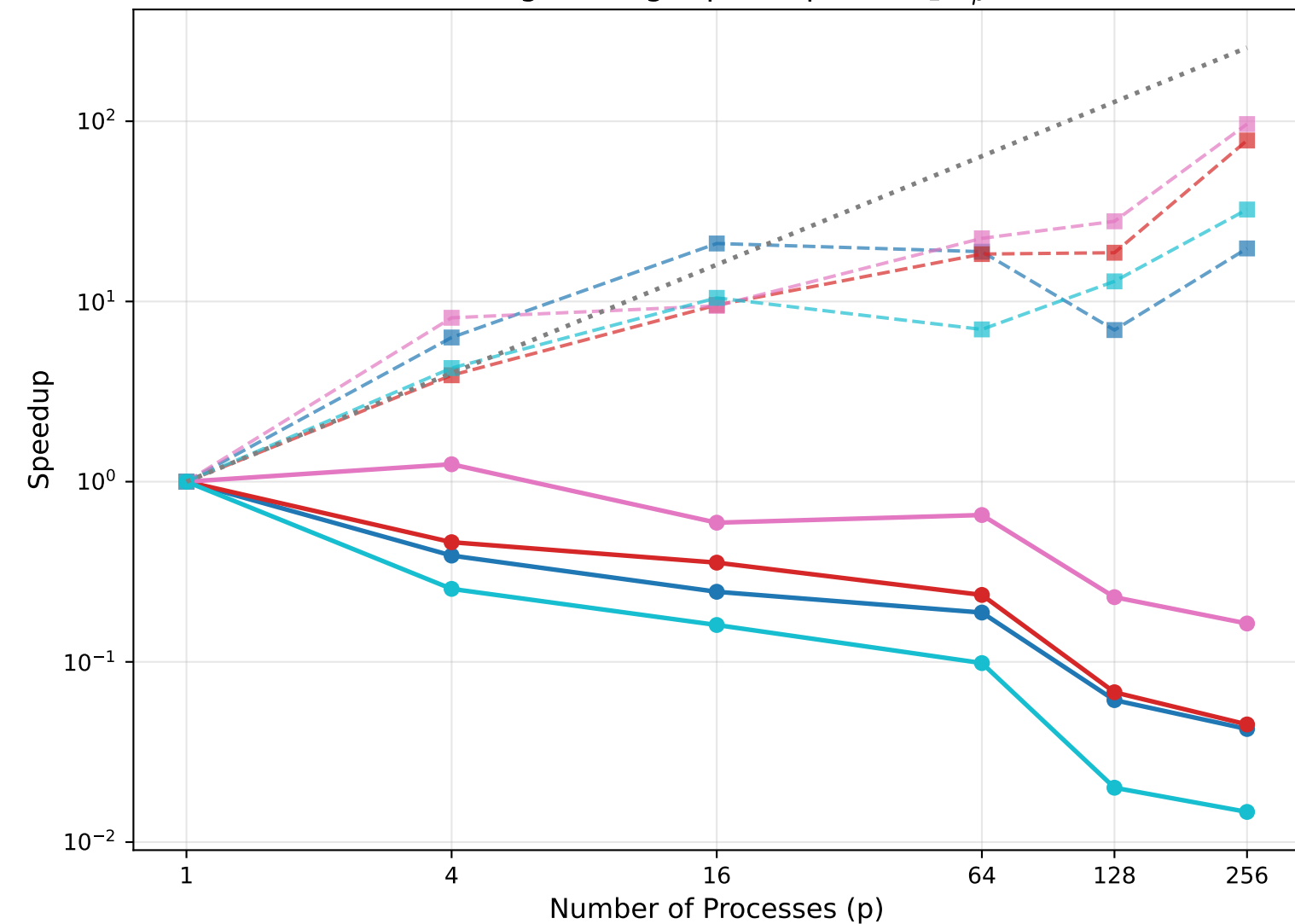
Strong Scaling: Speedup ( S = T_1/T_p )
