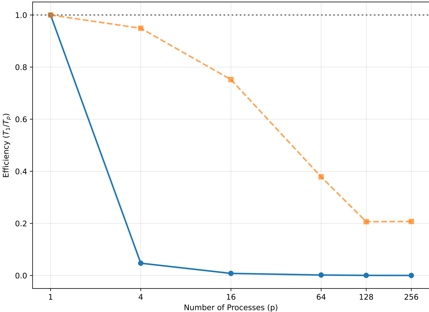
Weak Scaling: Efficiency
