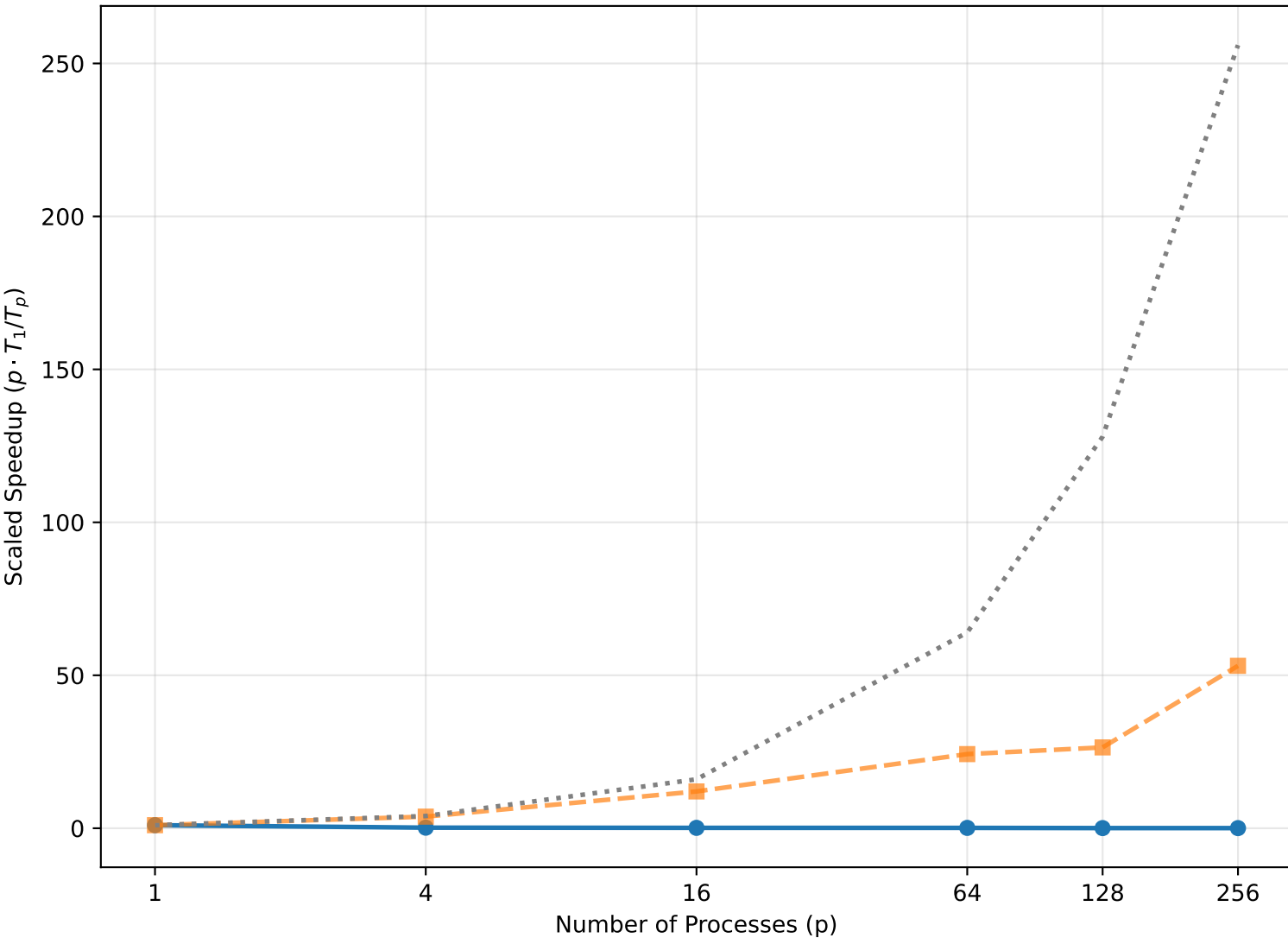
Weak Scaling: Scaled Speedup (Gustafson)
