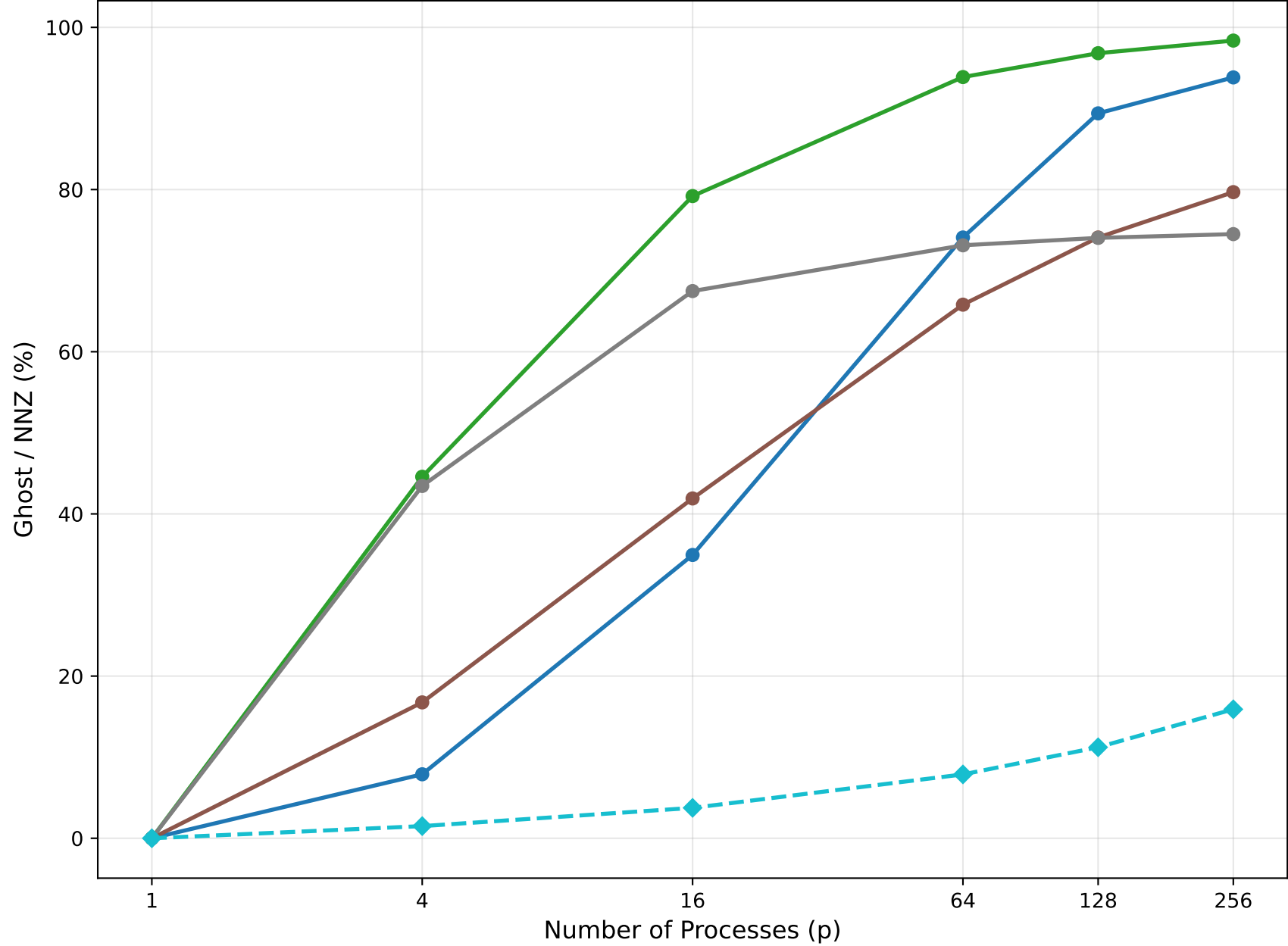
Communication Overhead (Ghost / NNZ)
