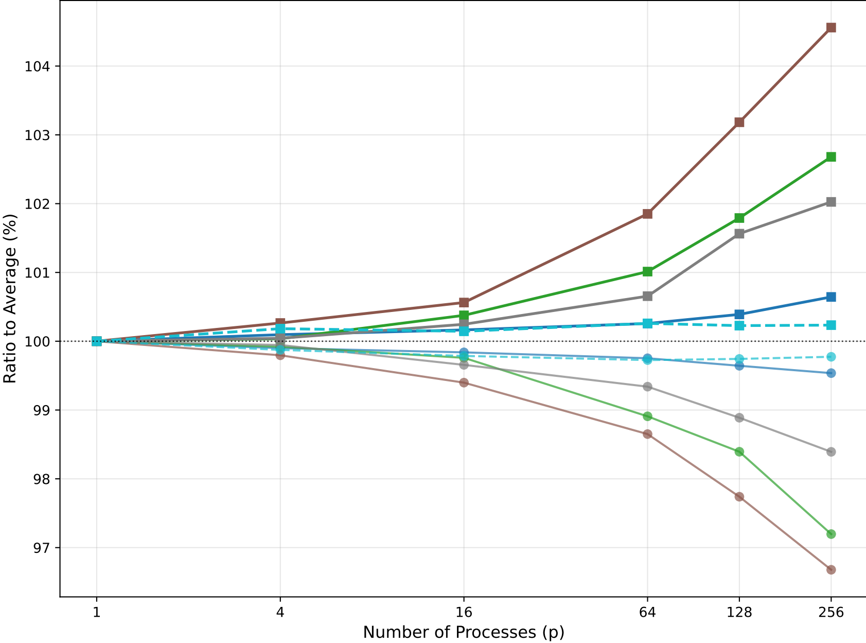
Load Balance: Min & Max vs Average NNZ
