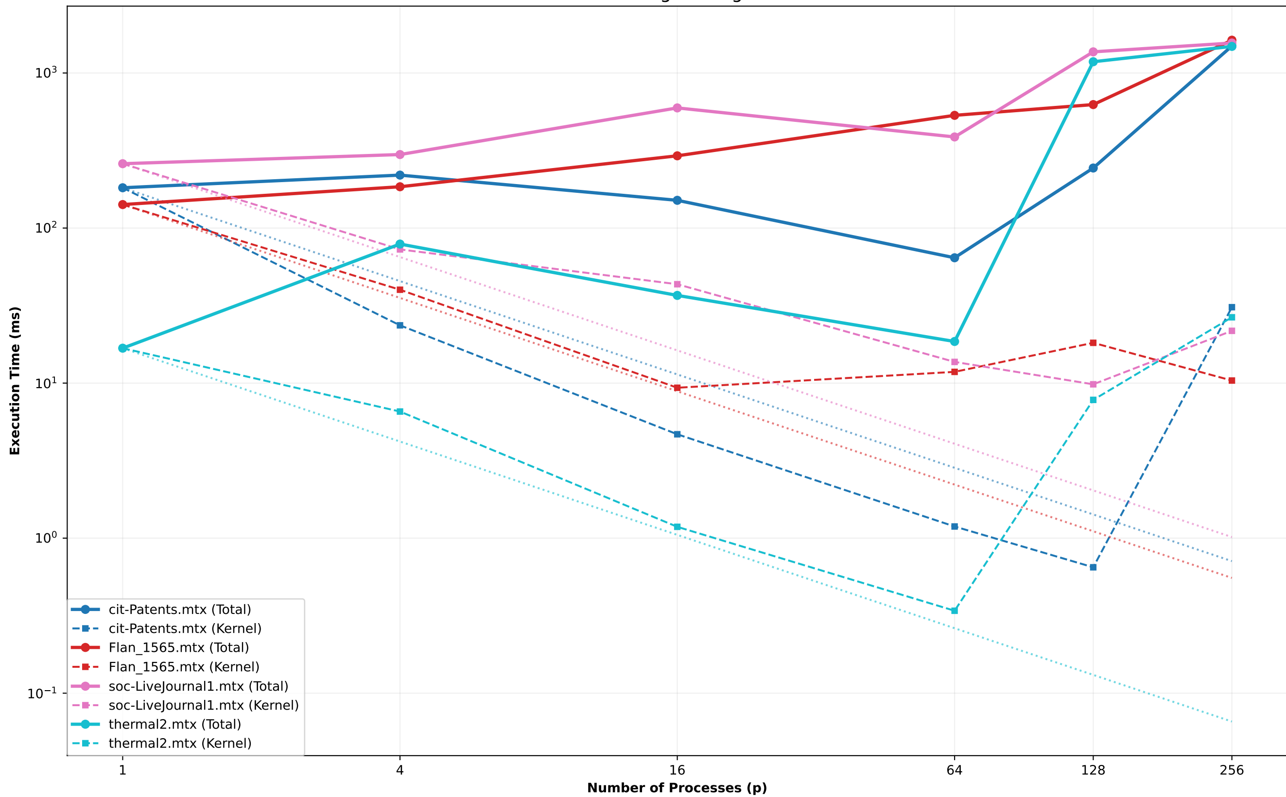
Strong Scaling
