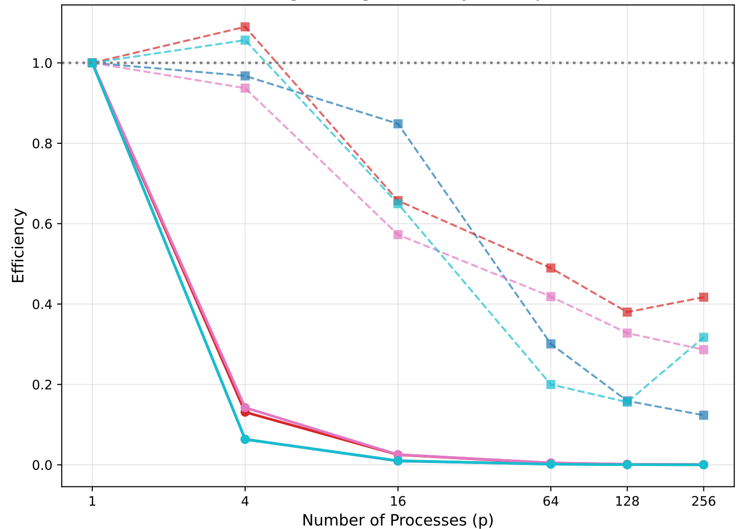
Strong Scaling: Efficiency ( E = S/p )
