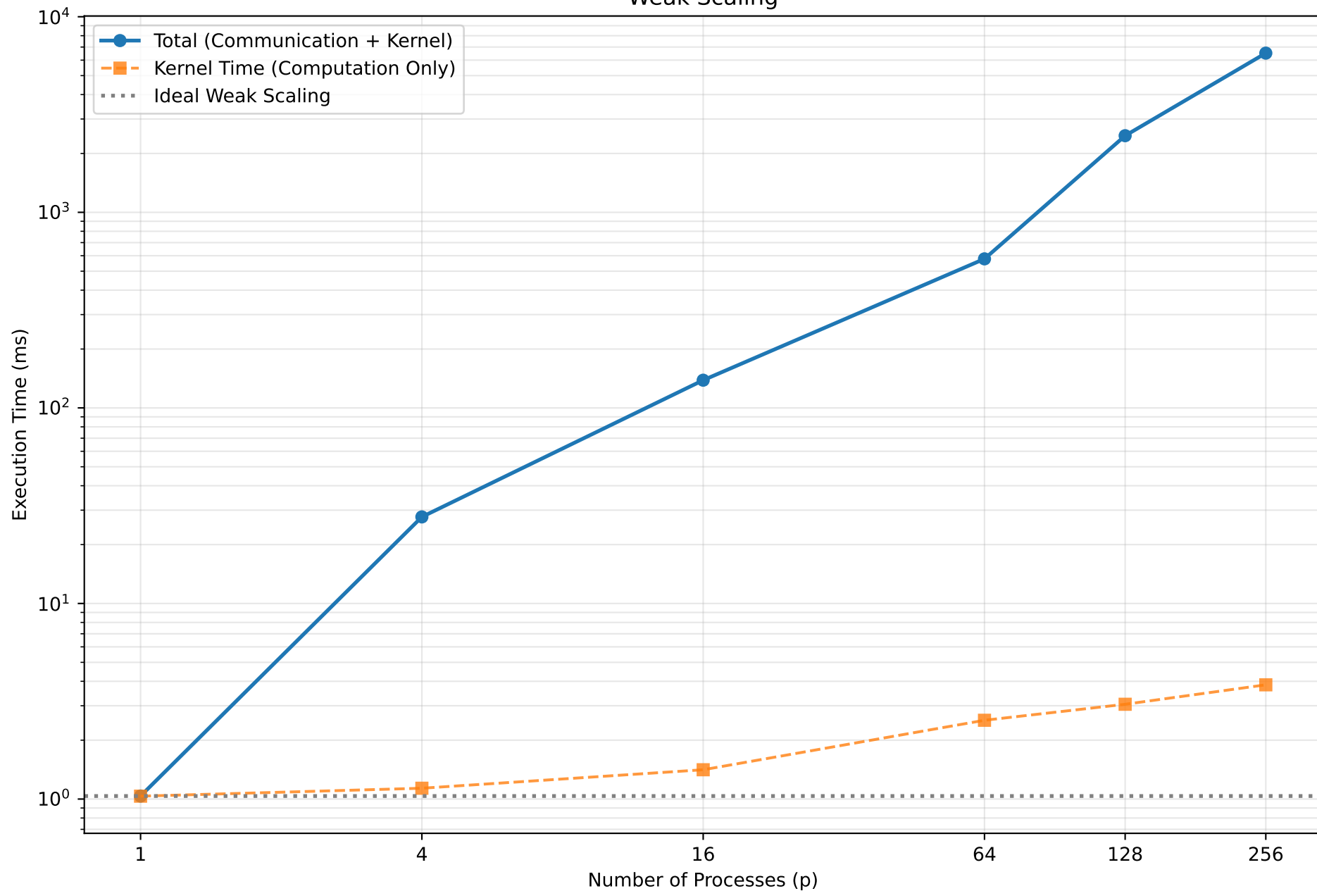
Weak Scaling
