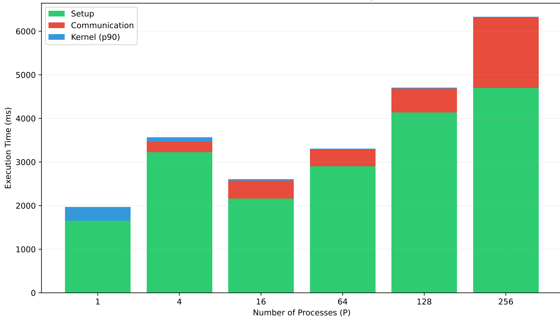
Execution Breakdown: ./matrices/soc-LiveJournal1.mtx
