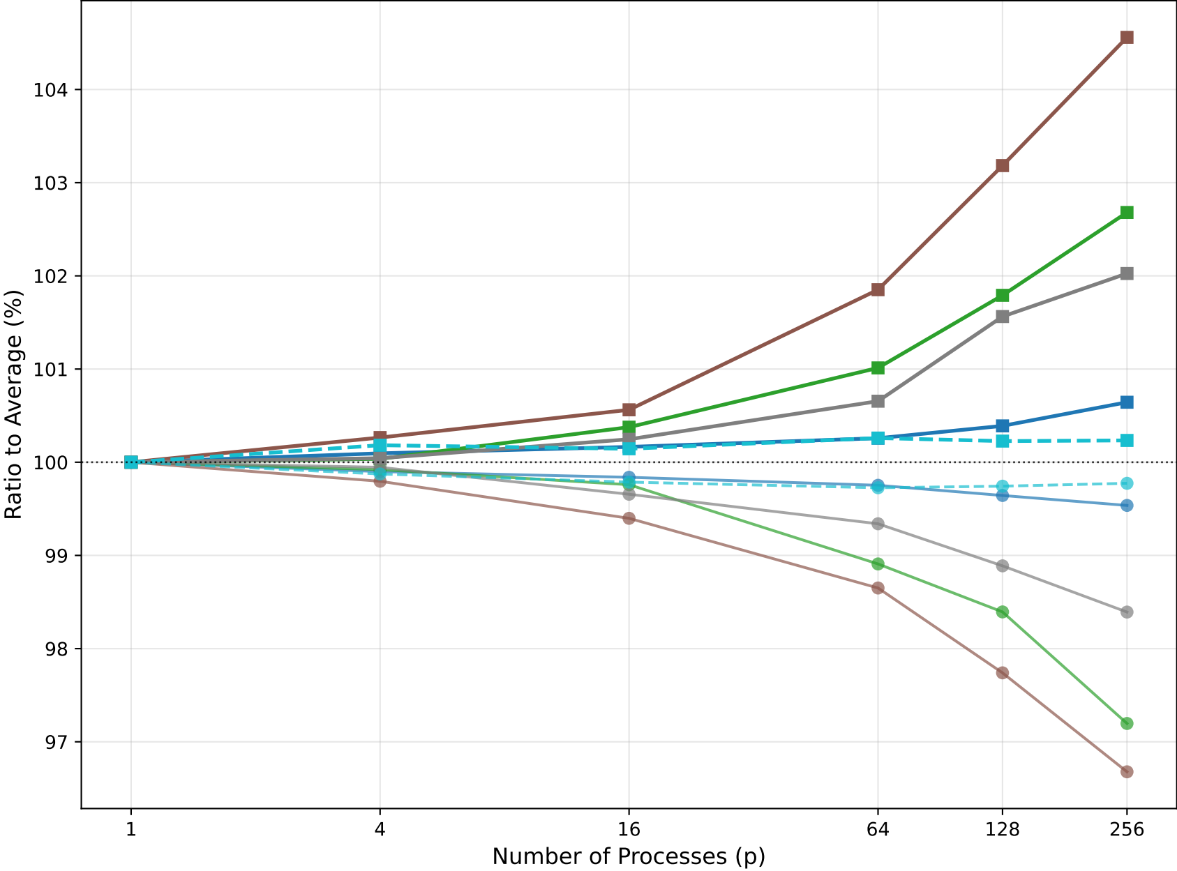
Load Balance: Min & Max vs Average NNZ
