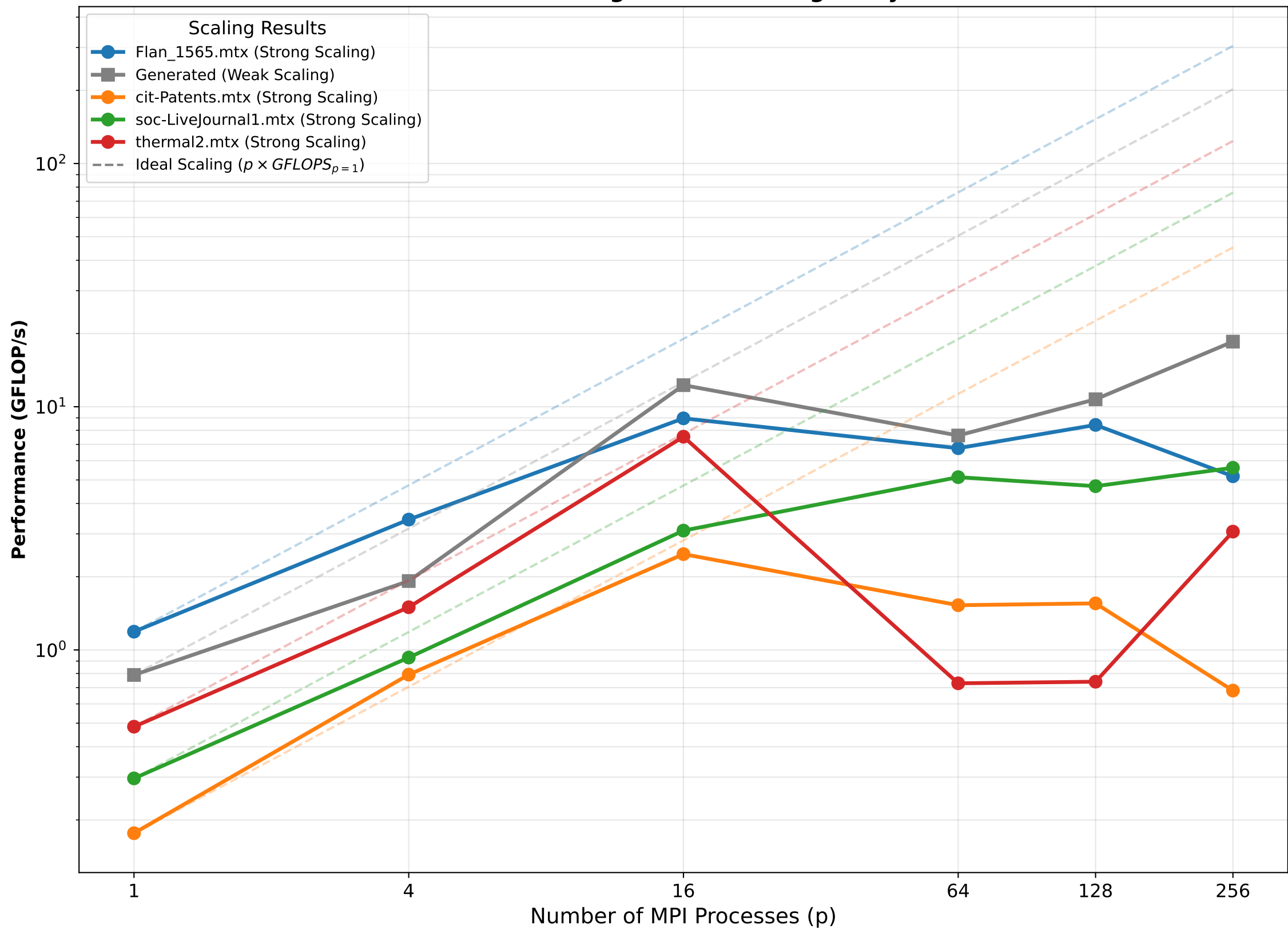
GFLOP/s Strong & Weak Scaling Analysis
