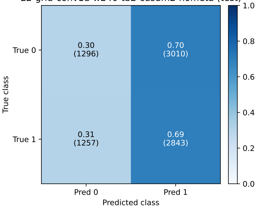
E2-grid-conv1d-w240-tb2-cusum2-nometa (test)
