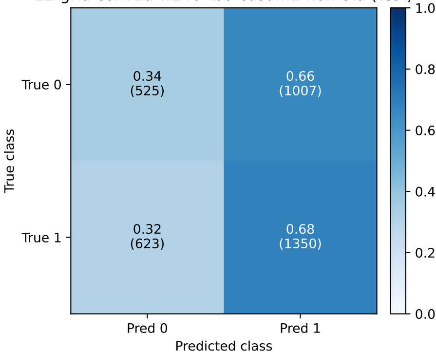
E2-grid-conv1d-w240-tb6-cusum1-nometa (test)
