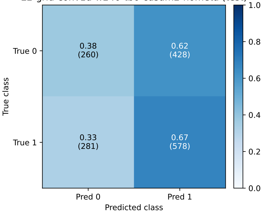
E2-grid-conv1d-w240-tb6-cusum2-nometa (test)
