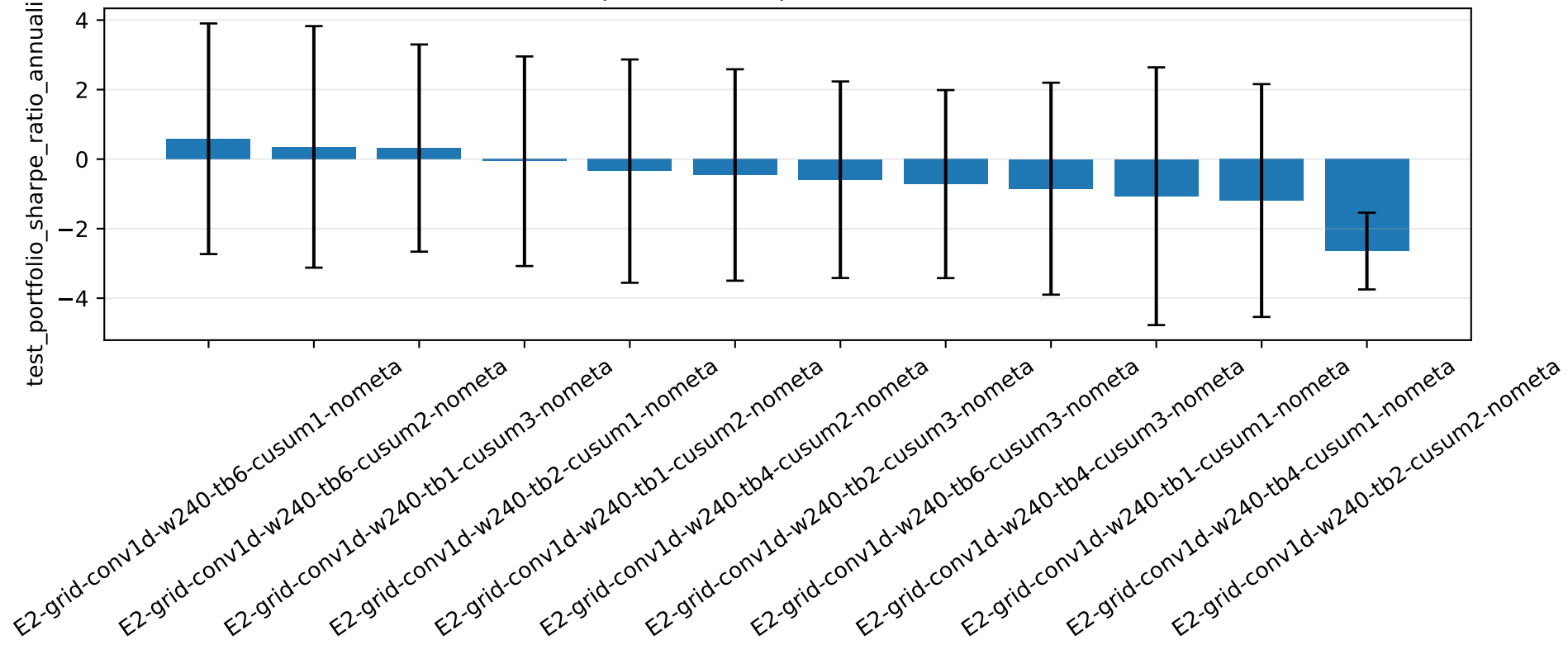
test portfolio sharpe ratio annualized
