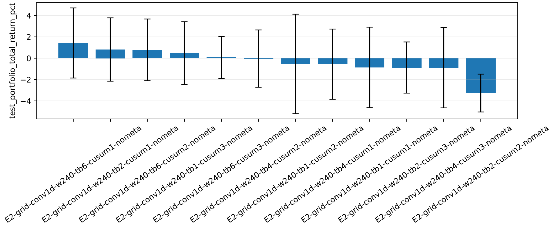
test portfolio total return pct
