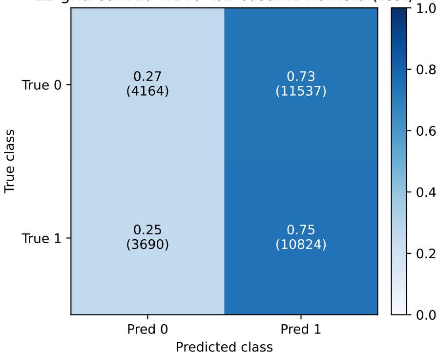
E2-grid-conv1d-w240-tb1-cusum1-nometa (test)
