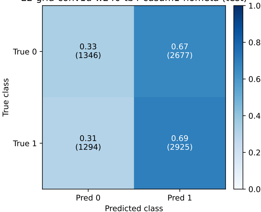
E2-grid-conv1d-w240-tb4-cusum1-nometa (test)
