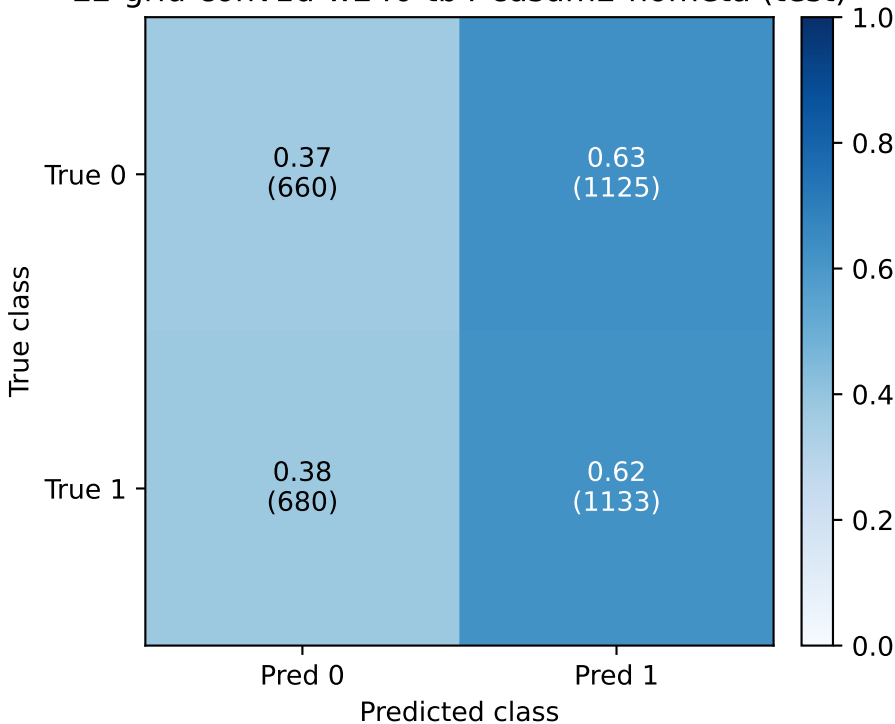
E2-grid-conv1d-w240-tb4-cusum2-nometa (test)
