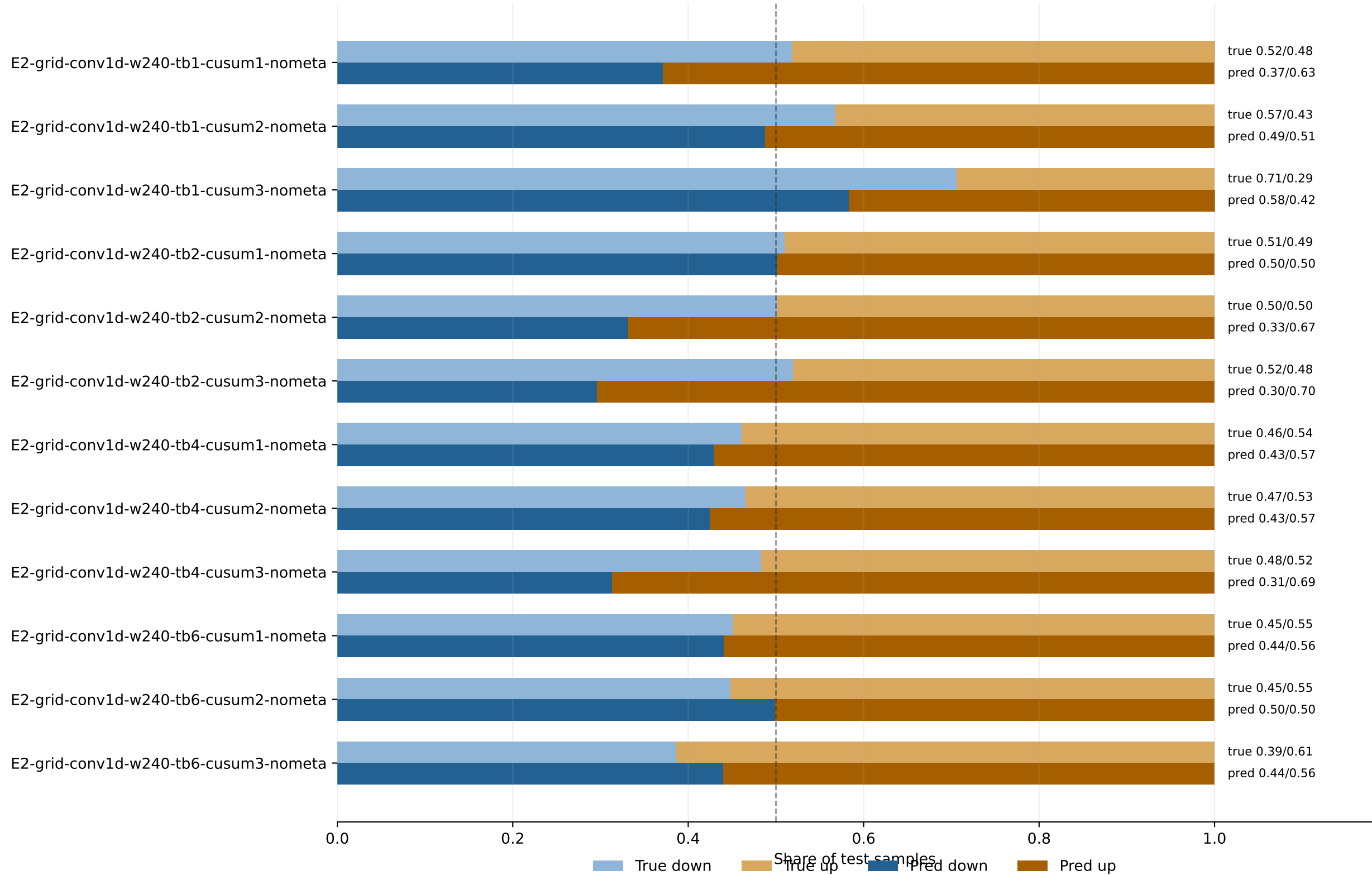
Test True vs Predicted Class Distribution
