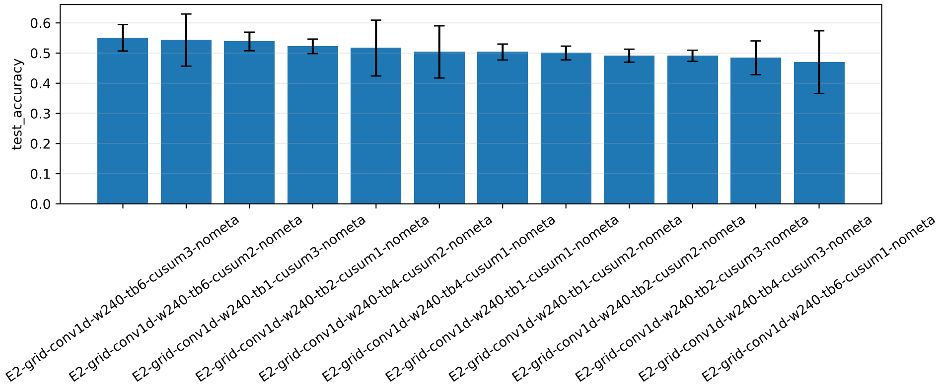
test accuracy
