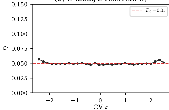
(b) D along x recovers D_0
