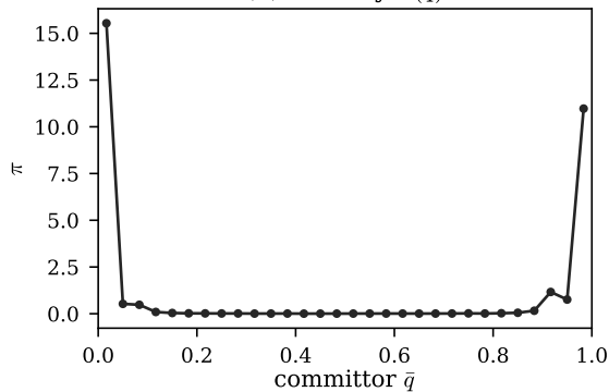
(a) Density \pi(\bar{q})
