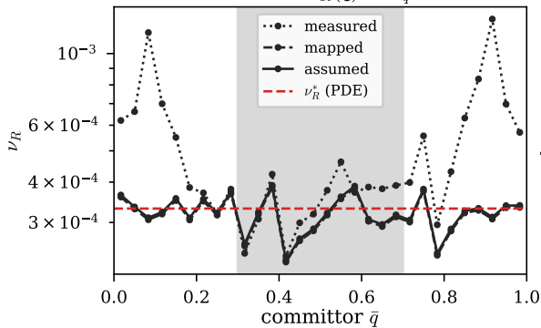
(c) Flux \nu_R(\bar{q}) = D_q \pi
