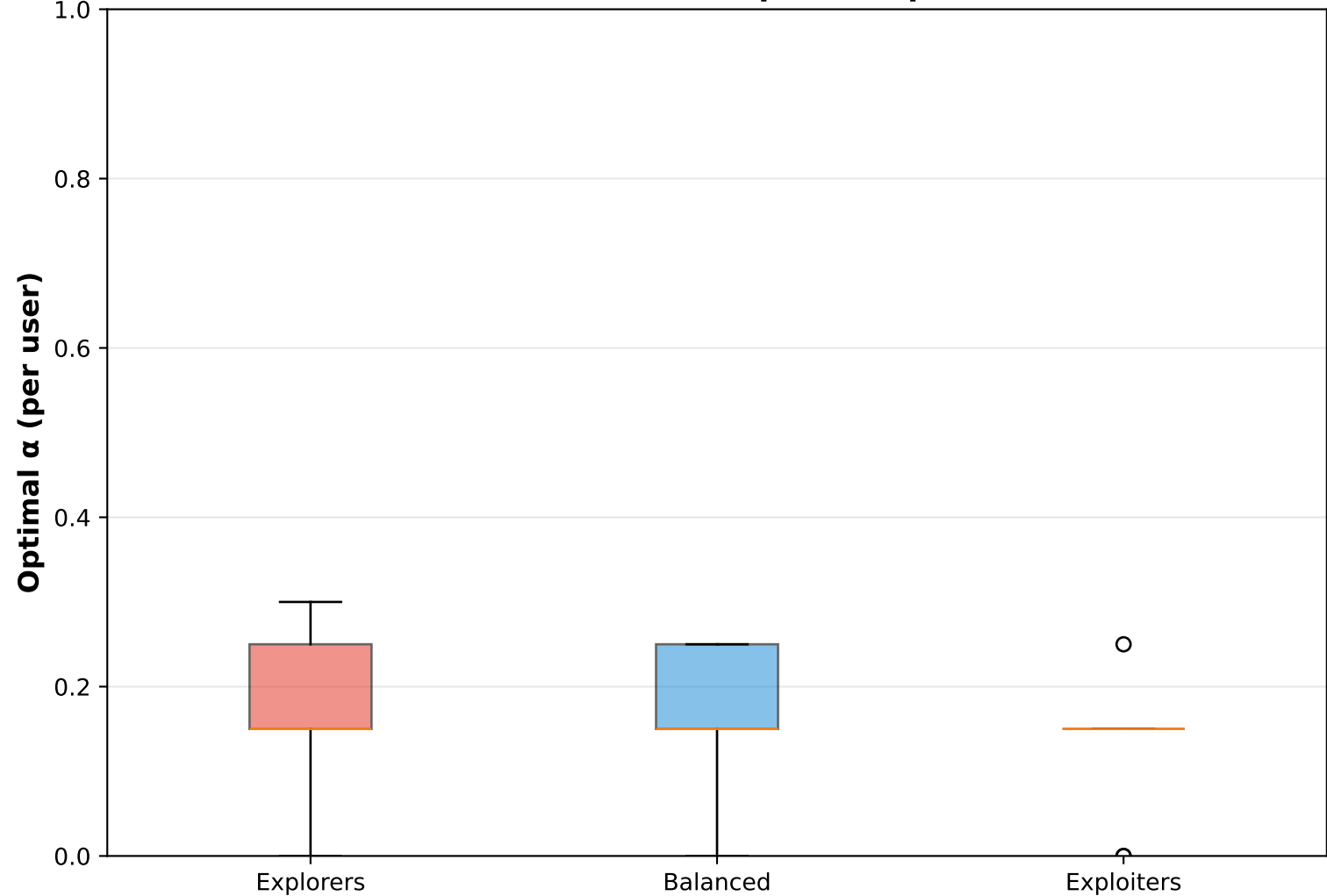
Distribution of User-Specific Optimal \alpha
