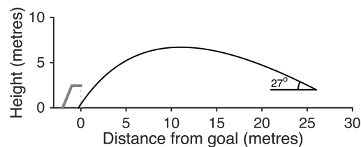
Figure 5.4 Aerodynamics of Zlatan Ibrahimović's bicycle lob, including drag.
