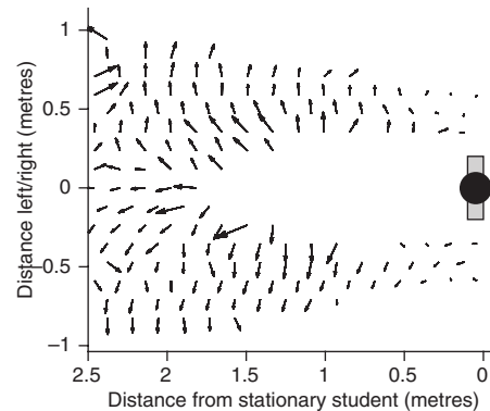
Figure 3.4 The effect a stationary student (positioned on the right of the figure) has on a student walking toward them in a corridor. Each arrow is the average reaction of the moving student to the presence of the stationary student. An upward-pointing arrow indicates a tendency to pass the stationary student on the left, while a downward-pointing arrow indicates a tendency to pass on the right. Adapted from original figure by Mehdi Moussaïd. 3
