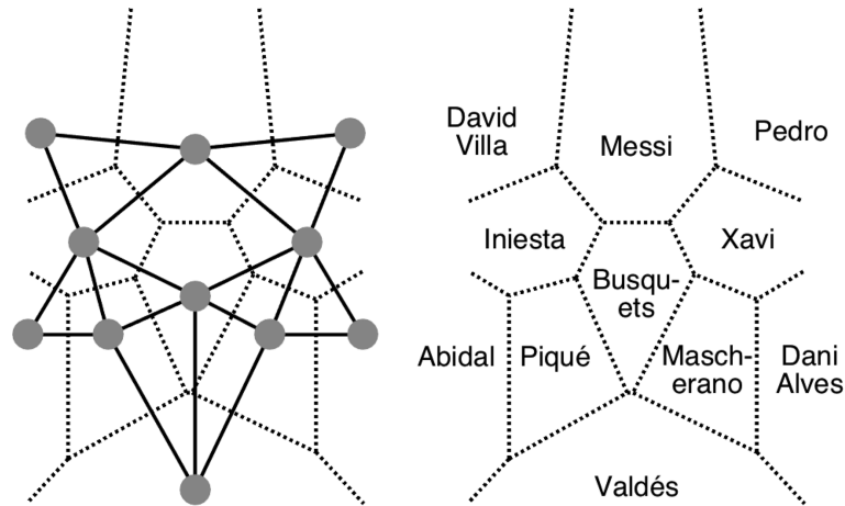
Figure 2.4 The Barcelona 2010/11 network and zones. The formation network (solid lines) together with the zones (dotted lines) for each player (left); typical position for each player during the season (right).
