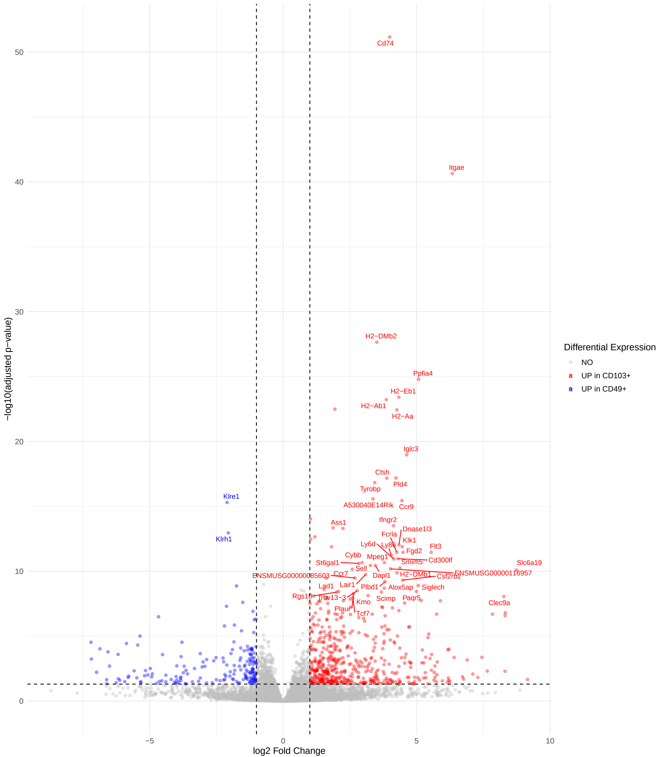
CD103+ stem-like vs CD49+ effector
