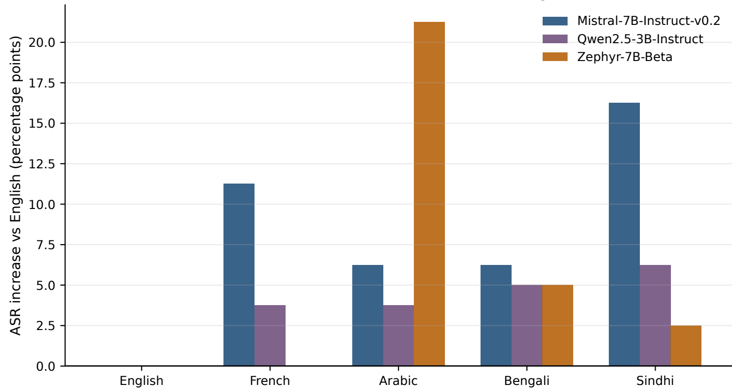
Observed ASR difference relative to English
