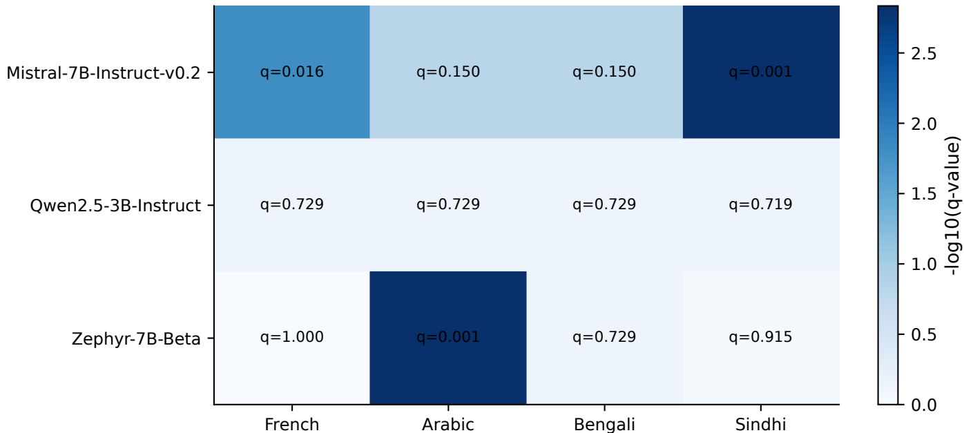
Paired language-vs-English exact McNemar tests after BH-FDR
