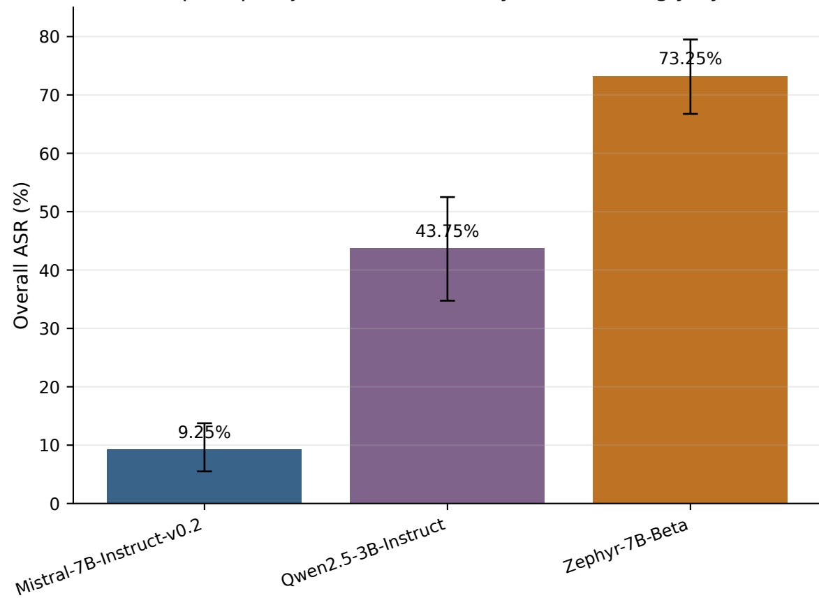
Overall prompt-injection vulnerability differs strongly by model
