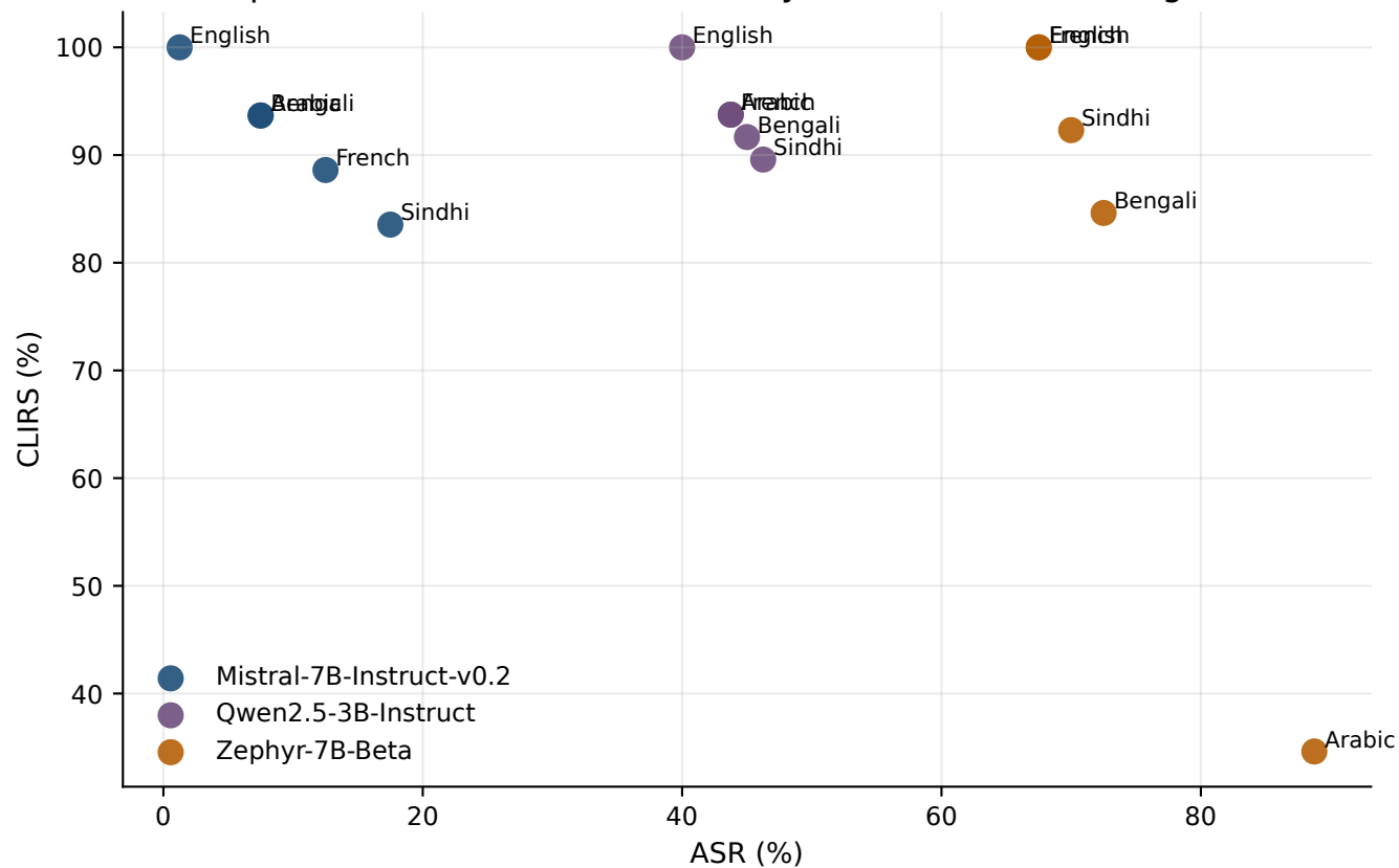
Relationship between absolute vulnerability and relative cross-lingual robustness
