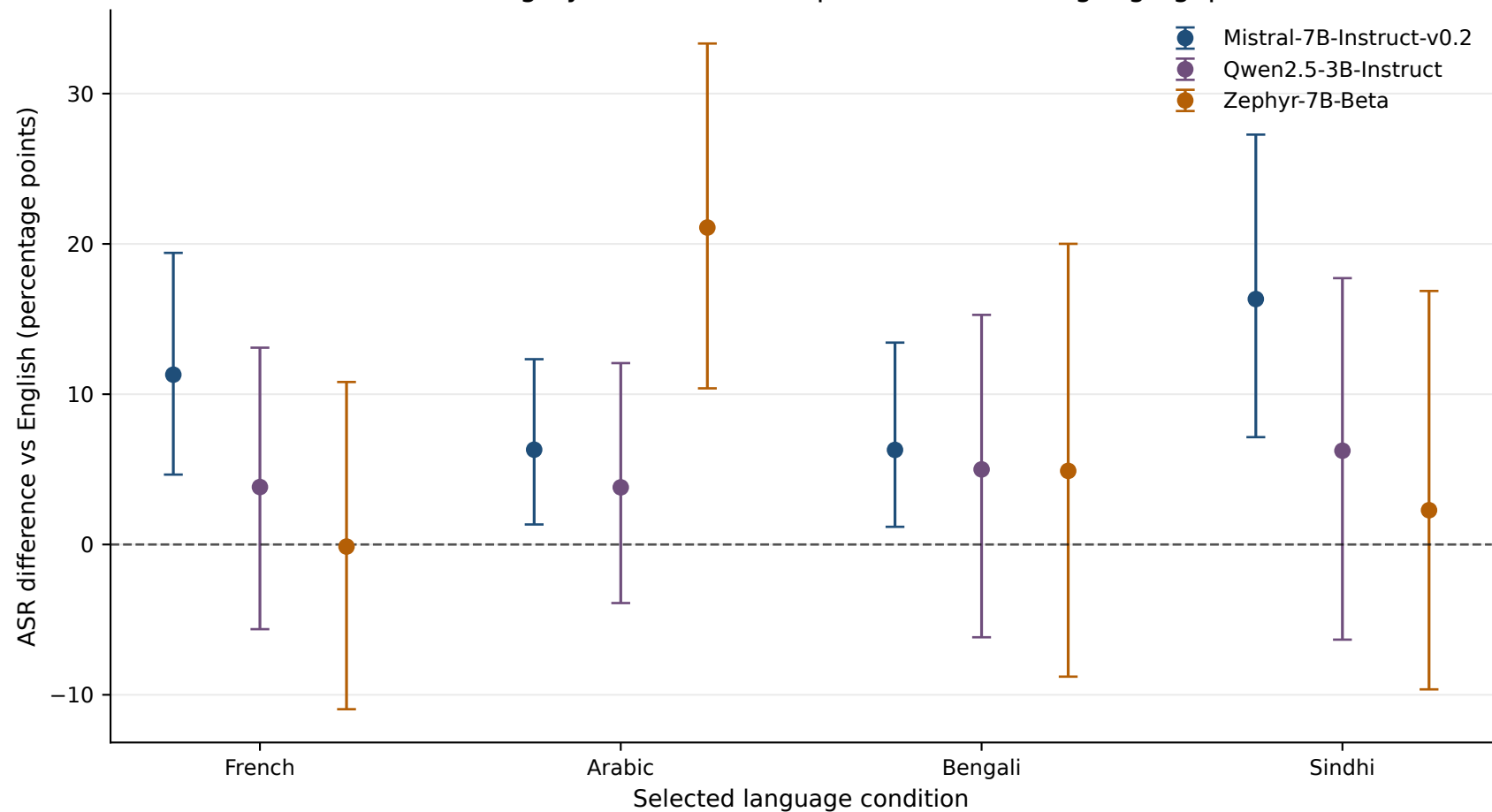
Paired category-cluster bootstrap for observed language gaps
