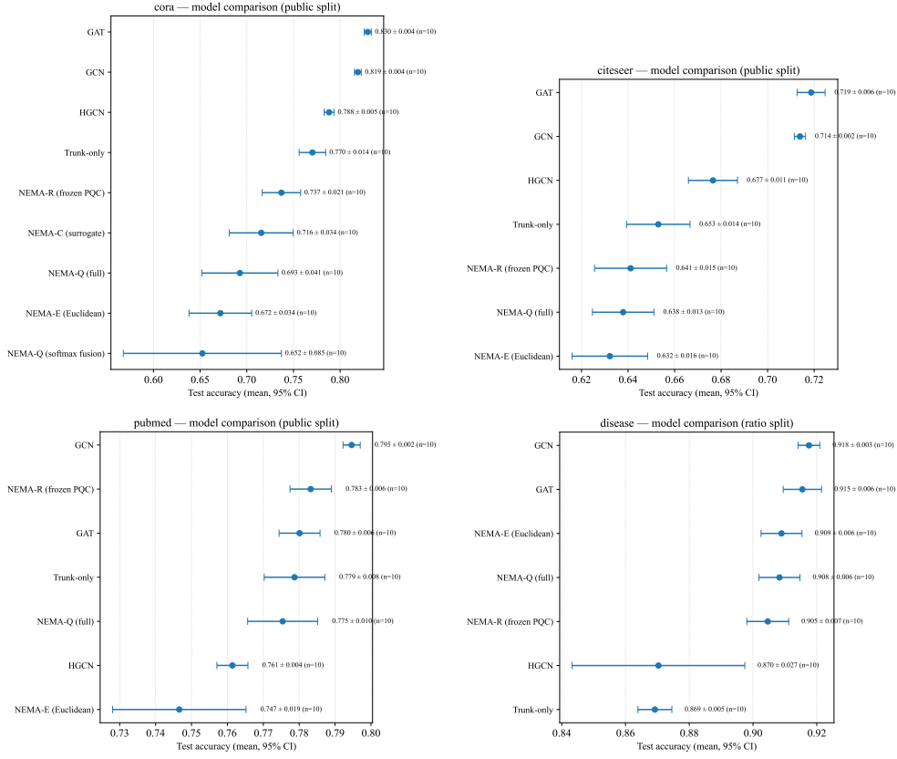
Fig. 4 Forest plots, one panel per dataset: test accuracy (mean \pm 95% CI over 10 paired confirmatory seeds) for all baselines, NEMA-Q, and every configuration-swap control under that dataset’s locked recipe.
