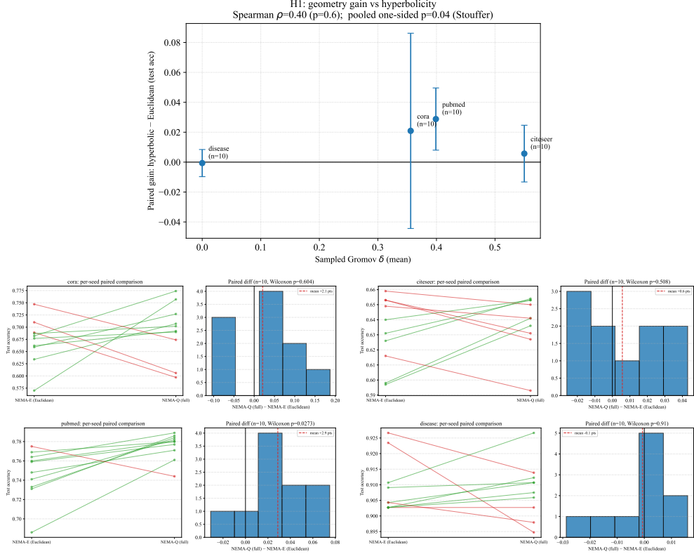
Fig. 7 Geometry \times \delta . Top: paired hyperbolic–Euclidean gain (mean \pm 95% CI) against dataset \delta_{\text{mean}} ; the preregistered H1(b) prediction is a negative slope, the observed trend is positive. The in-panel pooled annotation is the registered statistic (Stouffer over one-sided Wilcoxon tests). Bottom: per-dataset paired-seed plots (NEMA-Q vs. NEMA-E).
