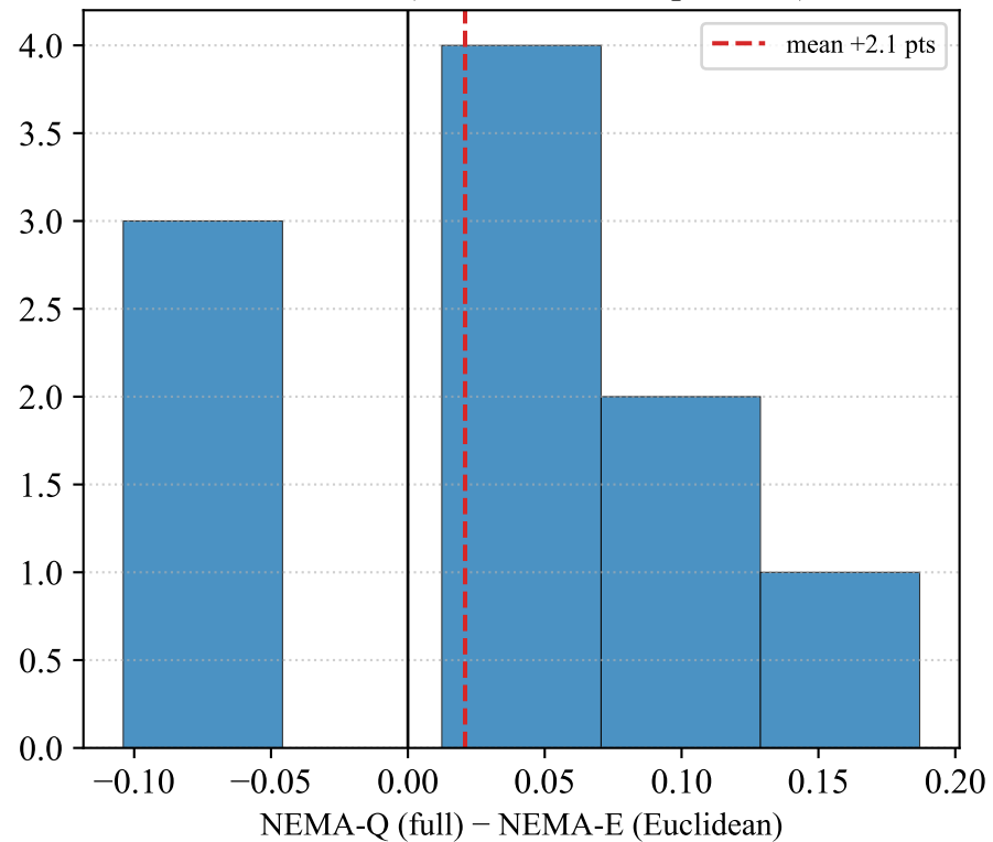
Paired diff (n=10, Wilcoxon p=0.604)
